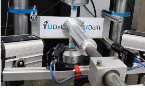
Figure 1. Experimental set-up.
