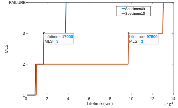
Figure 5. MLS diagnostic measure of testing specimens.
