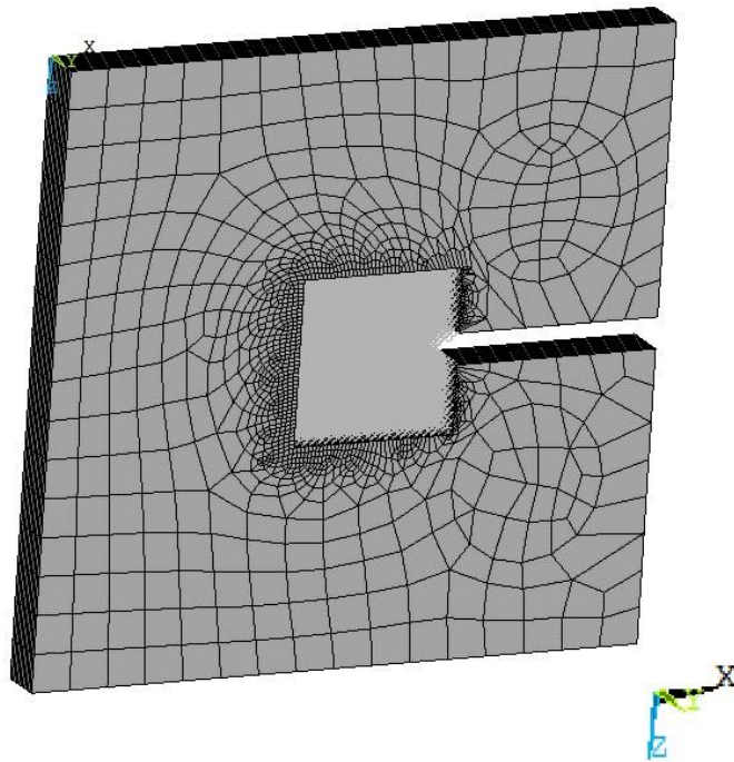
Figure 5- (a) A 3D view of the multi-scale FE model; (b) Implementation of extra cylinders to model the loading condition in the clamping area
