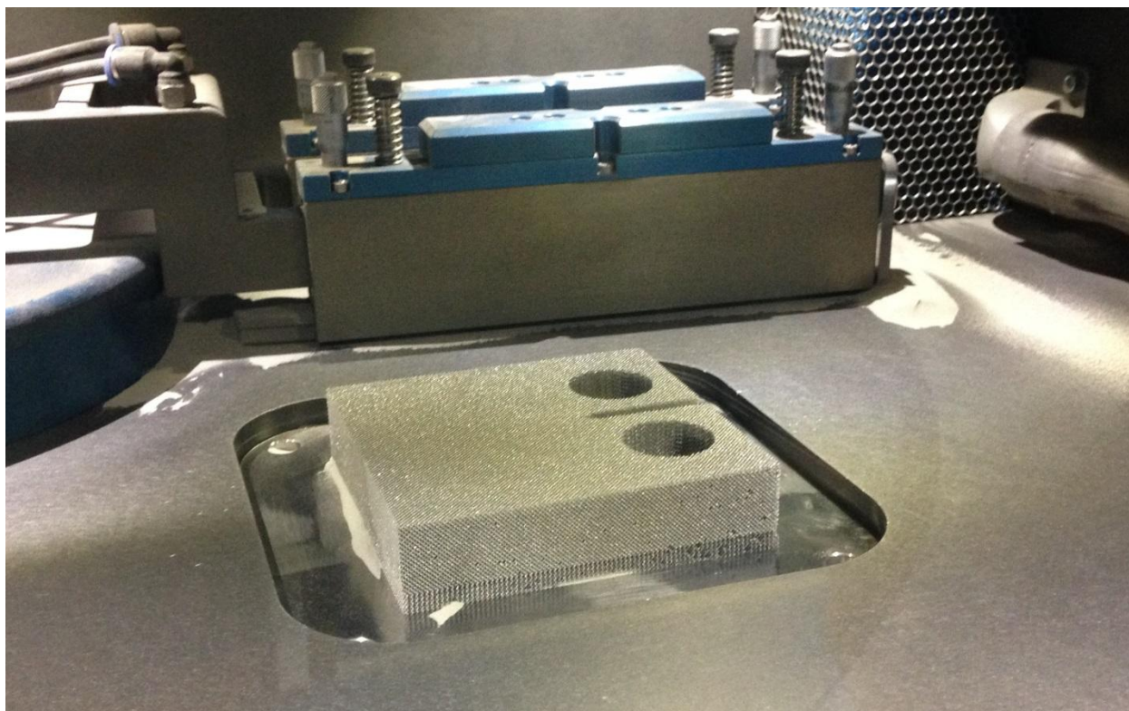
Figure 2- A view of the additively manufactured CT specimen in the SLM machine
