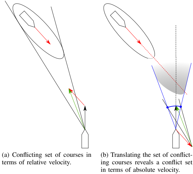
Figure 1. Derivation of the set of courses that lead to an intrusion, and the resulting conflict area.
