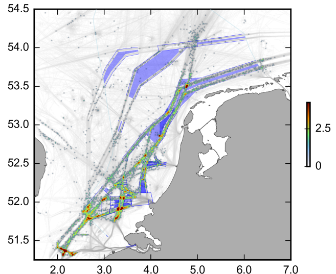
Figure 7. Conflict density of the area. A conflict requires a ship to manoeuvre within 450s to remain outside another ship's domain.
