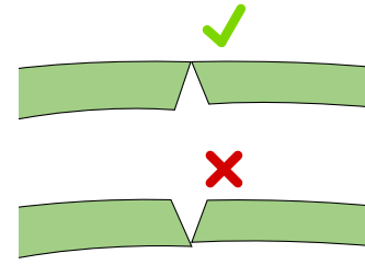
Figure 13: Thick panels might form a V-groove at their junction. To maintain continuity, the V-groove should be on the inner side of the track (top), rather than on the outer side (bottom).
