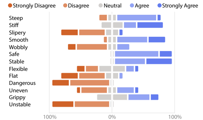
Figure 9: Summary of participant answers to our survey about their perception of the blade rollers.
