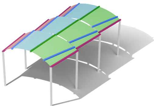
Figure 15: Bus shelter made of 3 arches, each composed of 4 wind turbine blade panels.
