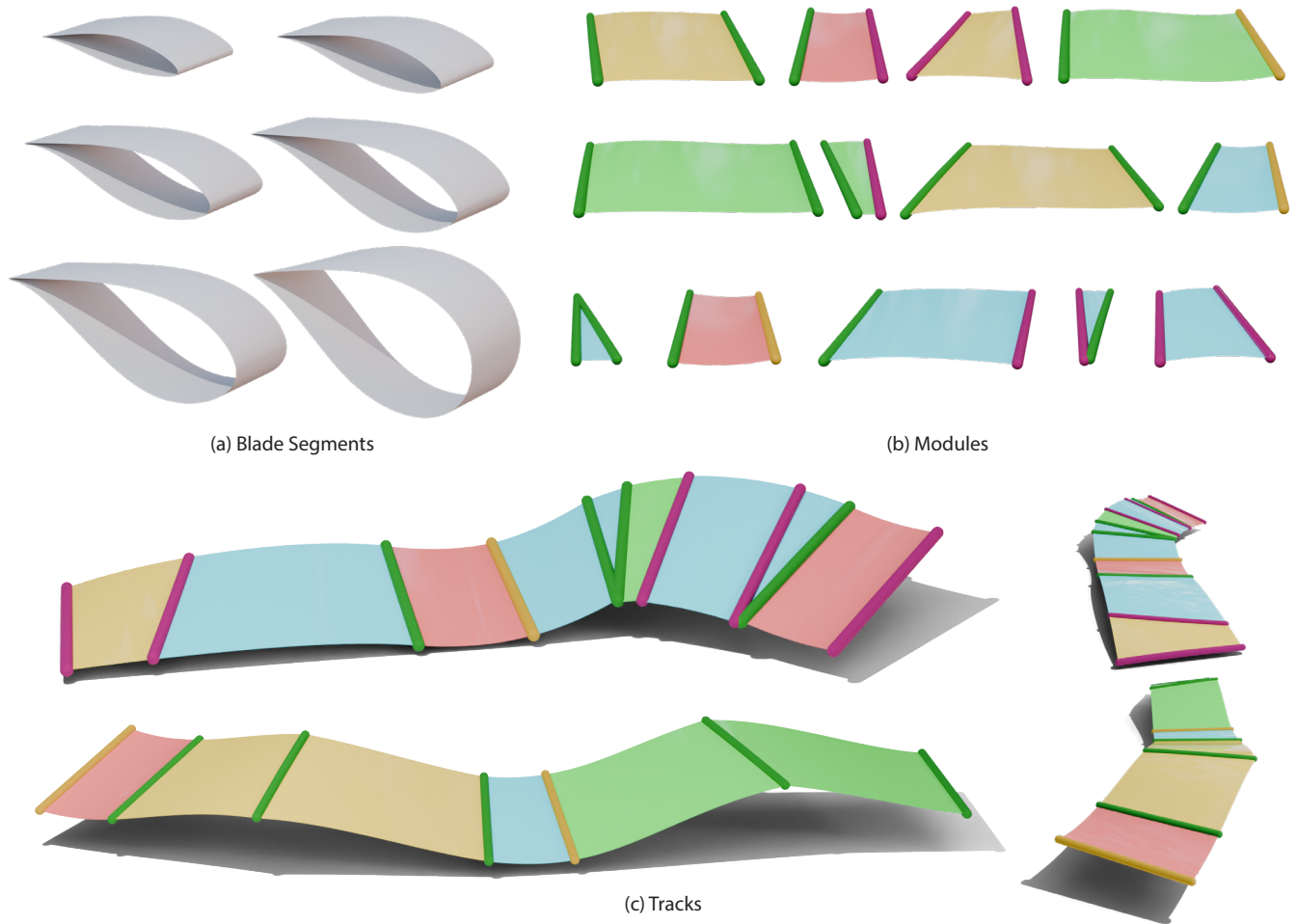
Figure 14: Taking 6 blade segments as input (a), our algorithm extracts 36 modules and identify 6 groups of compatible boundaries (b, only a subset of modules and compatibility groups shown). The modules exhibit diverse curvature, twist, and angle between their two extremities, allowing to create tracks with corners (c, top) and rollers (c, bottom).
