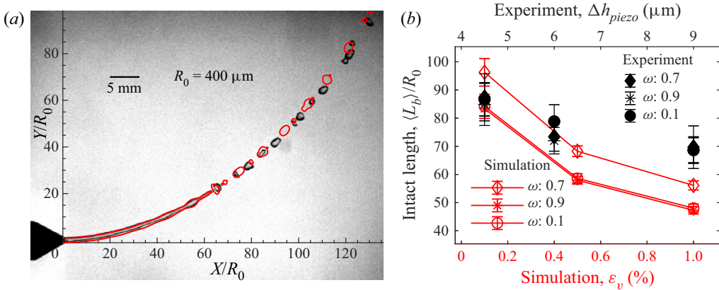
Figure 4. (a) Comparison of the jet interfaces obtained from simulation (shown in red) and from experiment at a perturbation frequency \omega = 0.7 . The piezoplate displacement is 6 \mu\text{m} and the velocity amplitude in the simulation is 0.5%. (b) Mean and standard deviation of the jet intact length as a function of piezoplate displacement in the experiments and velocity perturbation amplitude in the simulations.
