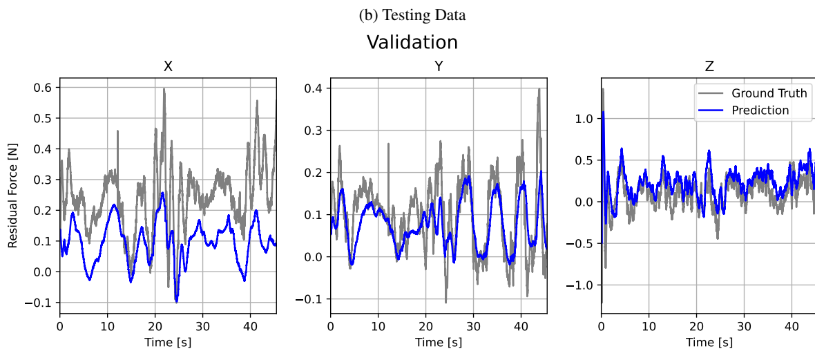
Figure 8: Unmodeled Force Predictions \hat{f}_{ext} = \phi(x) A^* for No Propeller Damage Condition
