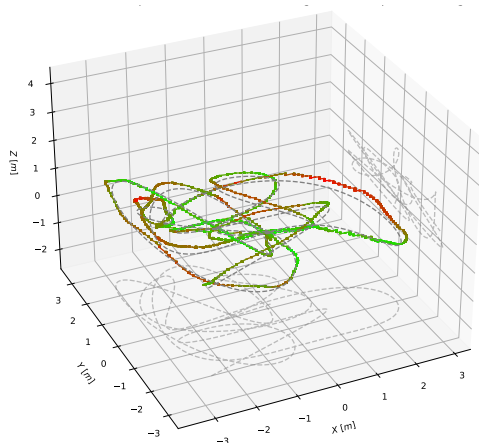
(e) Adaptive Neural Controller w/ Significant Propeller Damage
