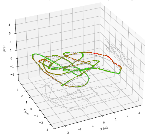
(a) Adaptive Neural Controller w/ No Propeller Damage
