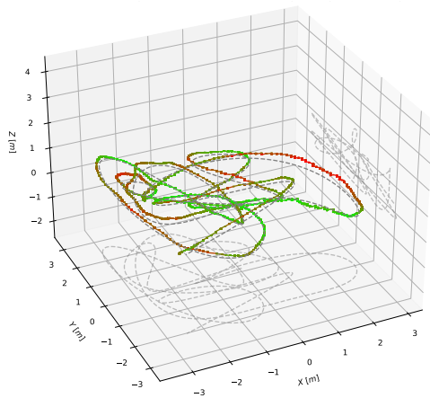
(c) Adaptive Neural Controller w/ Slight Propeller Damage
