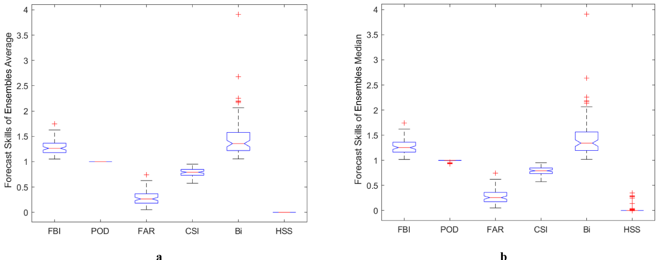
FIGURE 6 | Distributions of the forecast skill scores based on 87 stations (FBI, POD, FAR, CSI, Bi, HSS) for (a) average and (b) median of the ensemble members. [Colour figure can be viewed at wileyonlinelibrary.com ]
