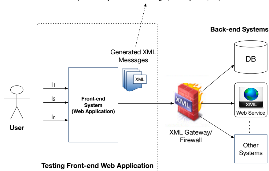
Fig. 1 An example of XML-based Enterprise System
