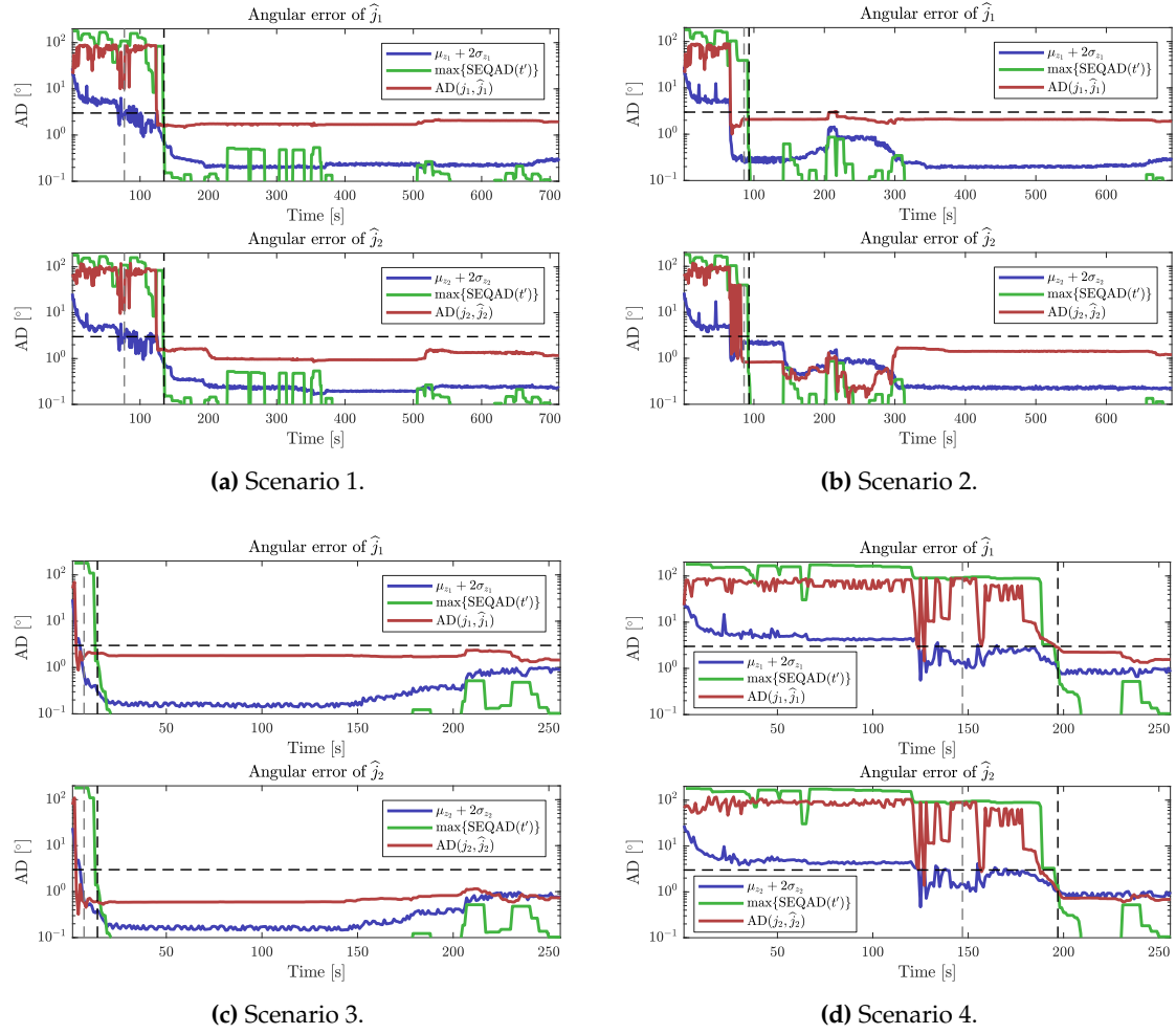
Figure 8. The plots show the local and global uncertainty metrics compared to the angular errors (red) for the four scenarios, see (a–d). Local uncertainty is quantified by \mu_z + 2\sigma_z , where \mu_z is the estimated mean AD (64) and \sigma_z is the standard deviation, computed from the estimated covariance matrix (65). Local uncertainty (blue) is shown for both \hat{j}_1 and \hat{j}_2 for each scenario. Global uncertainty is quantified by (68). The global uncertainty (green) with n_{\min} = 10 is shown for each scenario. Horizontal dashed lines show the accuracy threshold E_{\max} = 3^\circ . Vertical dashed lines show when estimates \hat{j} were accepted by Algorithm 4. For each scenario, the leftmost vertical lines show the case of n_{\min} = 3 and the rightmost vertical lines show the case of n_{\min} = 10 , where Algorithm 4 terminates when the estimates have reached the desired accuracy w.r.t. ground truth.
