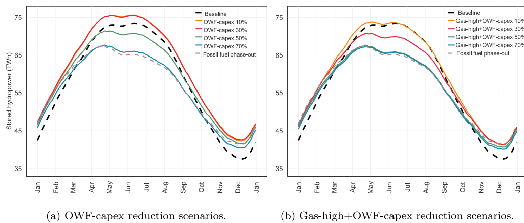
Fig. 18. Daily stored hydropower in TWh.
