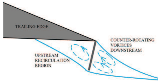
Fig 1: Mean flow field in the presence of a Gurney flap (reproduced from Liebeck, 1978)
