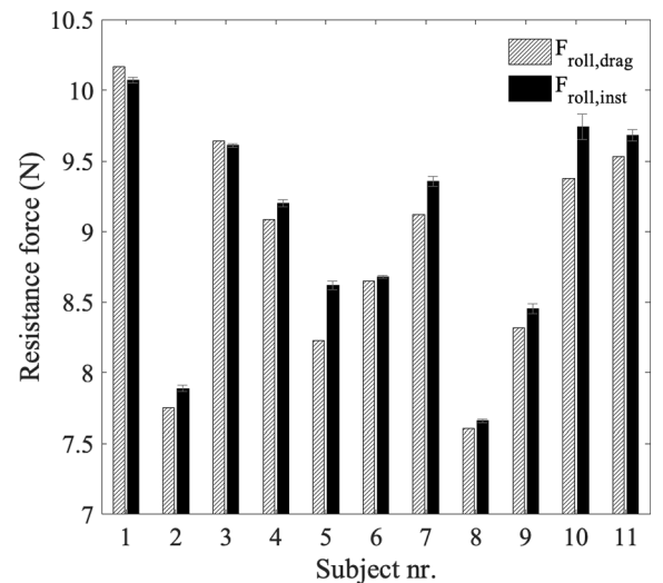
Fig. 5. (right) shows the differences between the resistance values of the drag test ( F_{roll,drag} ) and the average values + standard deviations of the instantaneous resistance force ( F_{roll,inst} ) for each participant. The measurements took place on a treadmill.
