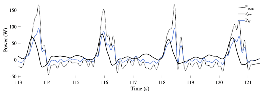
Fig. 3. Typical example of the instantaneous power graph of P_{AW} (black solid line), P_W (blue solidline) and P_{LMU} (black dotted line) of approximately four pushes at 1.2 m/s.
