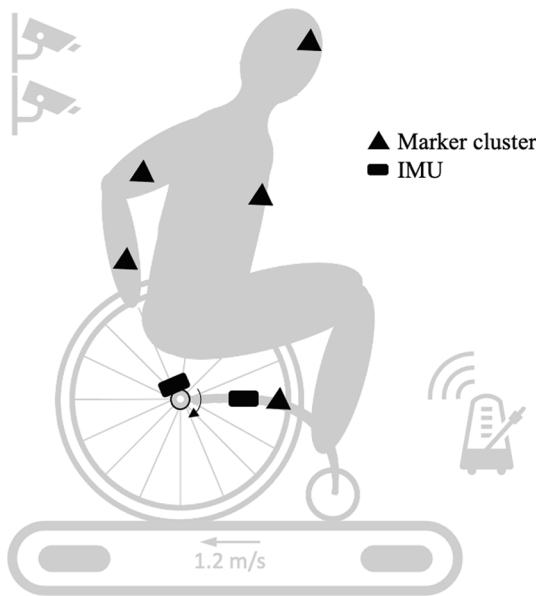
Fig. 2. Overview of the measurement setup. Participants were measured with a MOCAP system with marker clusters ( \Delta ) on the wheelchair frame, trunk (sternum), head, upper arm and lower arm, and IMUs ( \square ) on the wheel axle and on the center of the wheelchair frame. Both the 3.0 \times 5.0 m treadmill and the 1.0 \times 1.0 force plate (below the treadmill) are visible in the figure.
