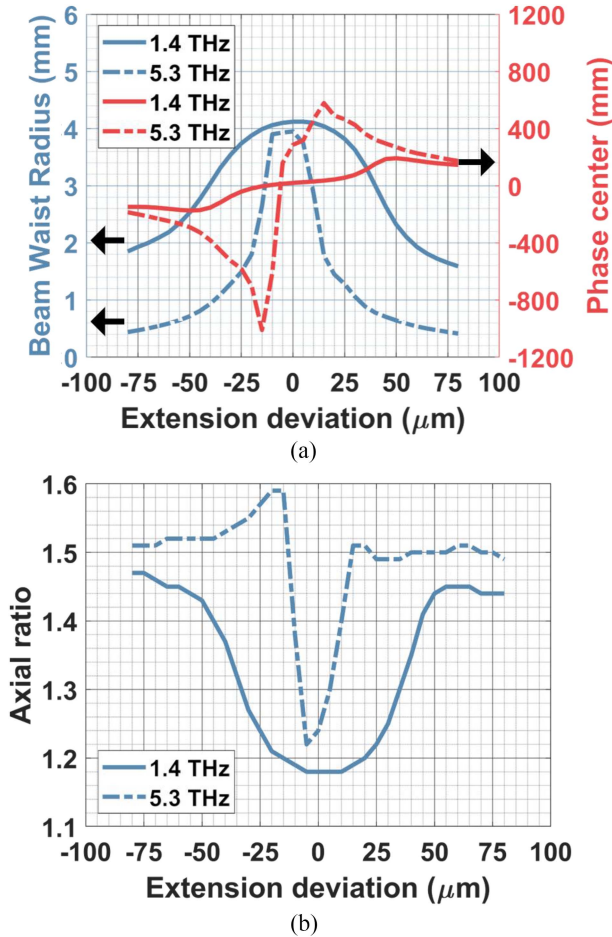
Fig. 5. Simulation results of the beam properties for a 10 mm diameter, elliptical lens by varying its extension deviation, at 1.4 and 5.3 THz. The nominal extension of the lens is 1550 \mu\text{m} . Calculated beam waist radius and phase center in (a), and axial ratio (b) are plotted as a function of extension.
