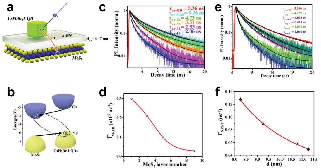
Figure 9. (a) Schematic and (b) band alignment of the monolayer MoS 2 and 8.5 nm sized CsPbBr 2 I nanocrystals HS studied by Luo and co-workers. (c) Room-temperature TRPL spectra of the HS with additional MoS 2 layers. (d) The corresponding non-radiative relaxation rate as a function of the increasing number of MoS 2 layers. (e) TRPL spectra of the HS with increasing hBN spacer thickness. (f) The corresponding non-radiative relaxation rate as a function of the hBN spacer thickness. [80] John Wiley & Sons. © 2019 WILEY-VCH Verlag GmbH & Co. KGaA, Weinheim.
