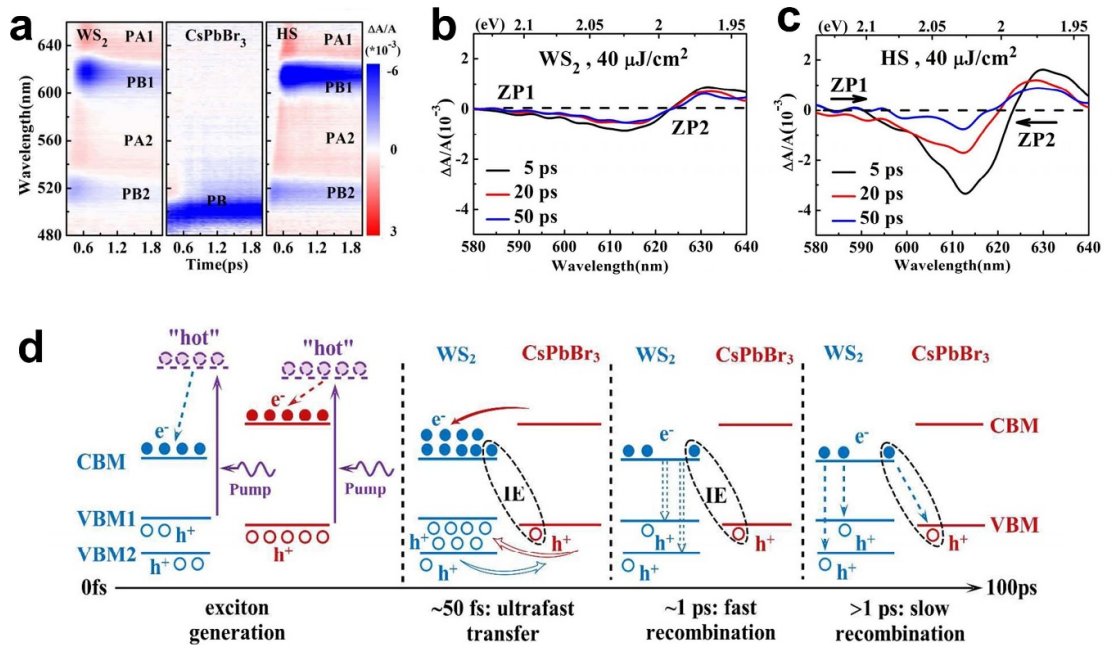
Figure 10. (a) Transient absorption spectroscopy with photobleaching (PB) and photo-induced absorption (PA) signals labelled for the monolayer WS 2 , 11 nm sized-CsPbBr 3 nanocrystals pristine samples and the WS 2 /CsPbBr 3 HS. PB1 (PB2) refers to the PB signals of the A (B) excitons. (b) TA signal of the A exciton resonance of the WS 2 structure. (c) TA signal of the A exciton resonance of the HS. Note the evolution of the ZP and the enhanced PA effect in the HS compared to the pristine sample. (d) Kinetic model of the ultra-fast charge processes of the HS. Reproduced from [184] with permission from the Royal Society of Chemistry.
