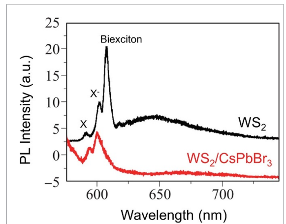
Figure 8. Low-temperature PL spectra of the WS 2 pristine sample and the WS 2 /CsPbBr 3 HS. The CsPbBr 3 consists of 180 nm thick microplates. Note the emission differences from the neutral exciton (X), the charged exciton (X − ) and the biexciton between the spectra. Reproduced from [101], with permission from Springer Nature.
