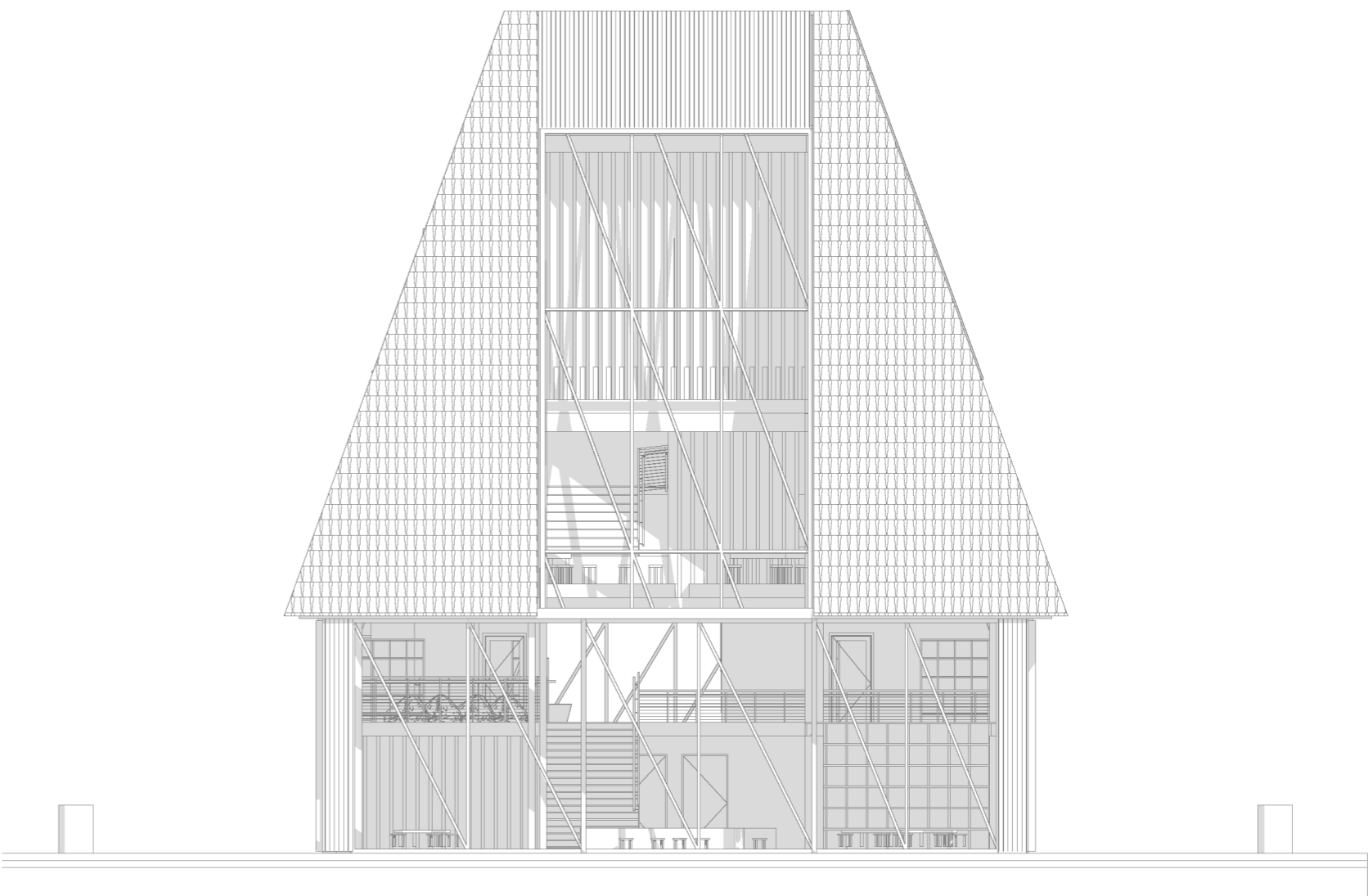
South Elevation
