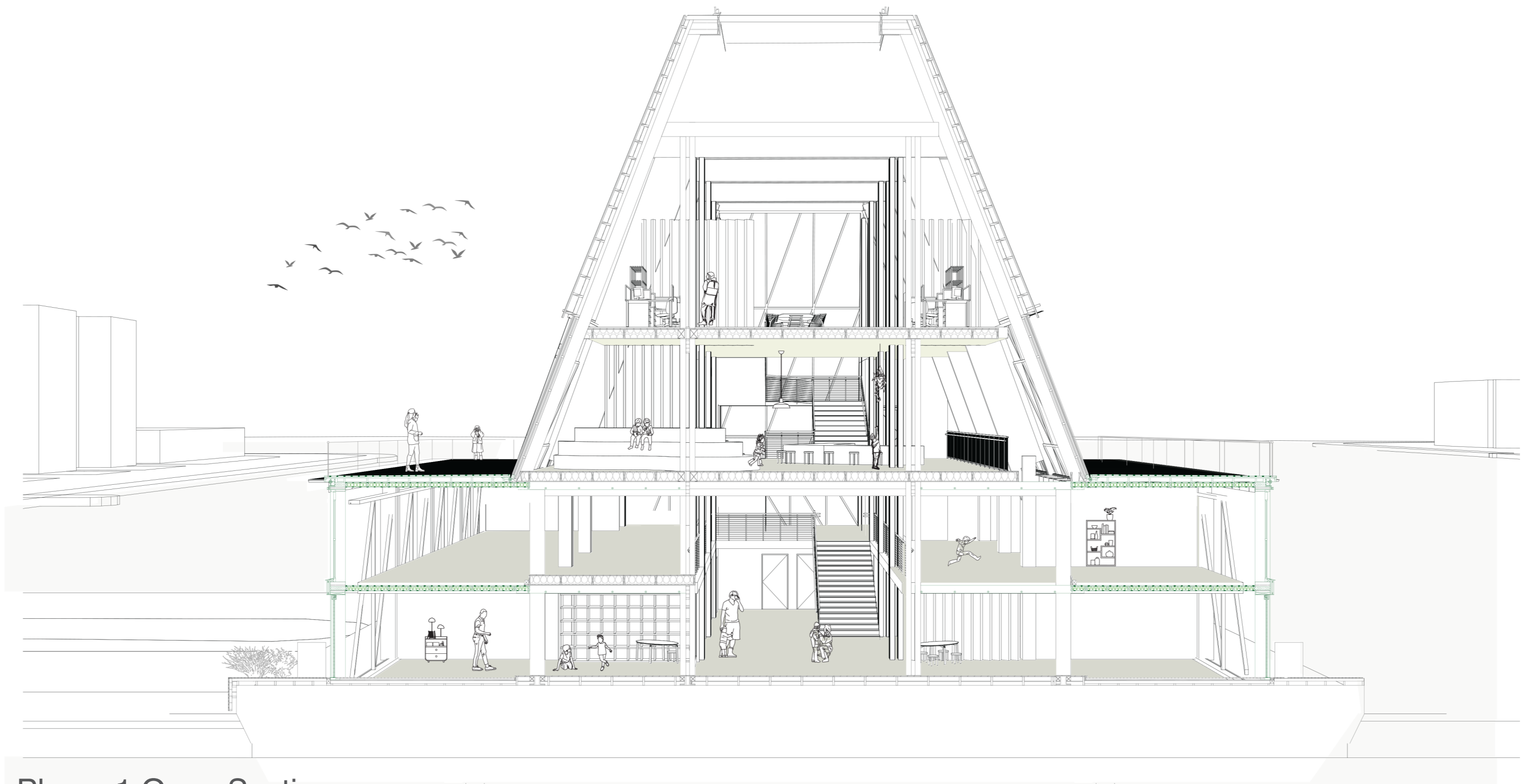
Phase 1 Open Section
