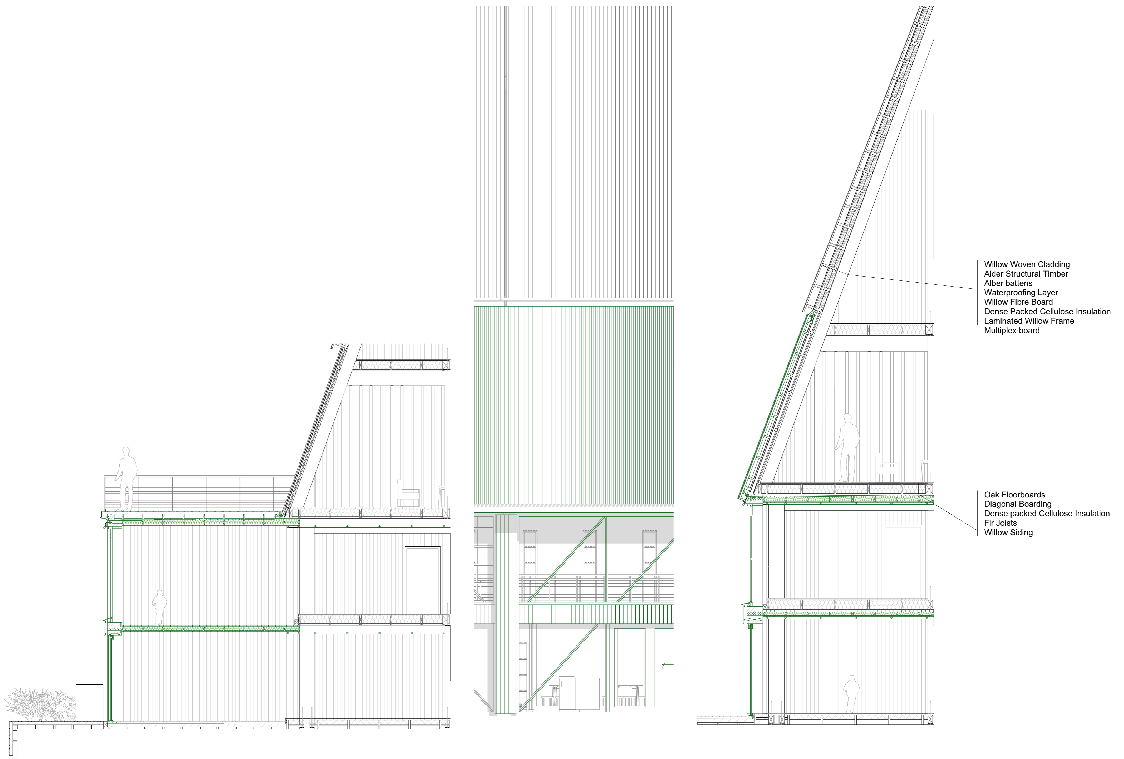
Expansion Scheme 1:50
