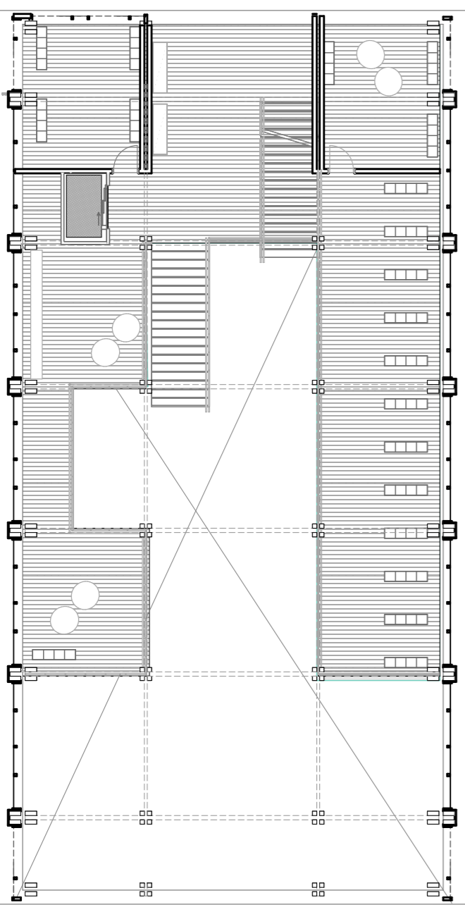
1st Floor
