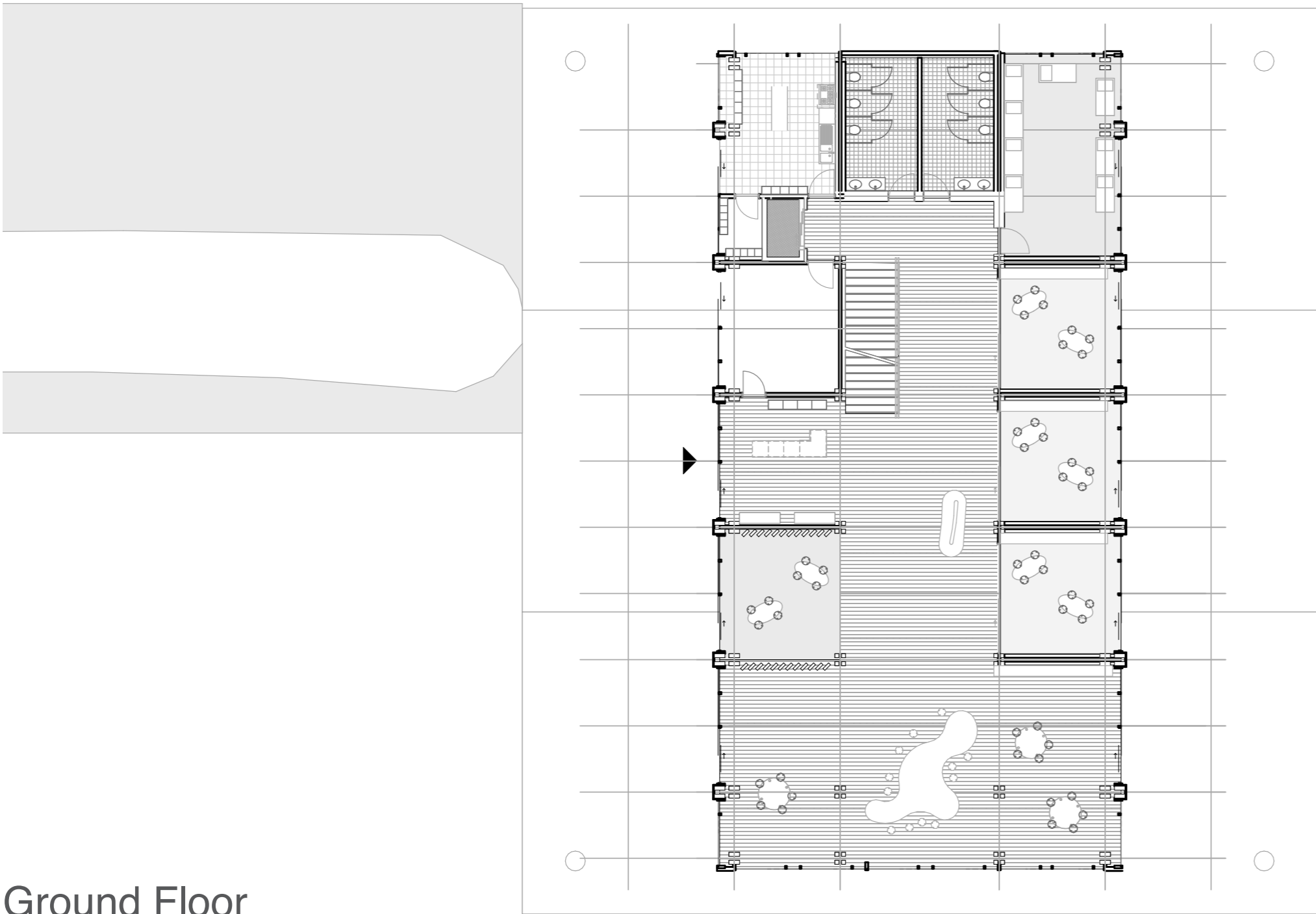
Ground Floor
