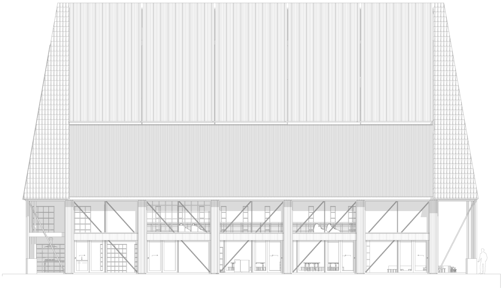
West Elevation
