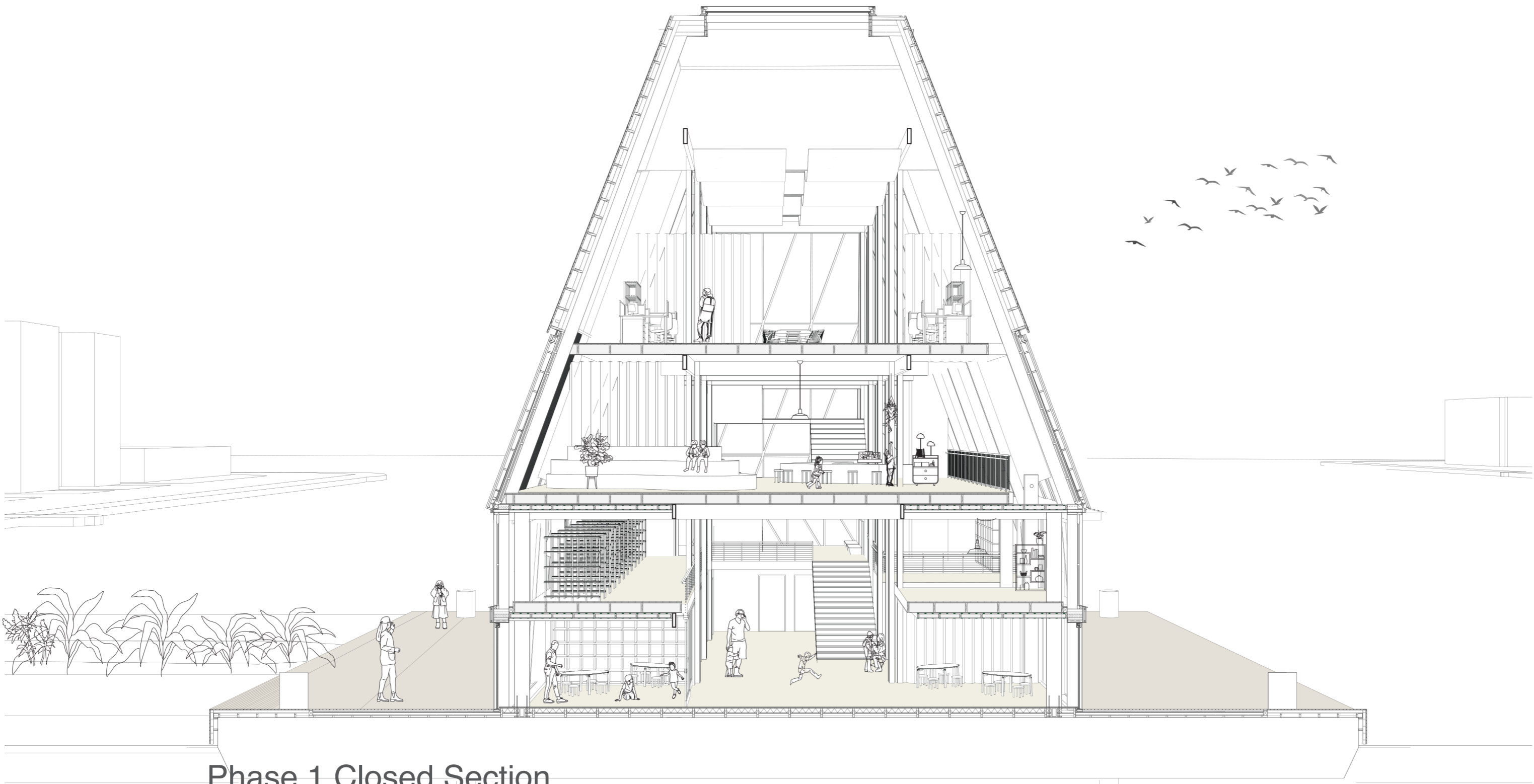
Phase 1 Closed Section
