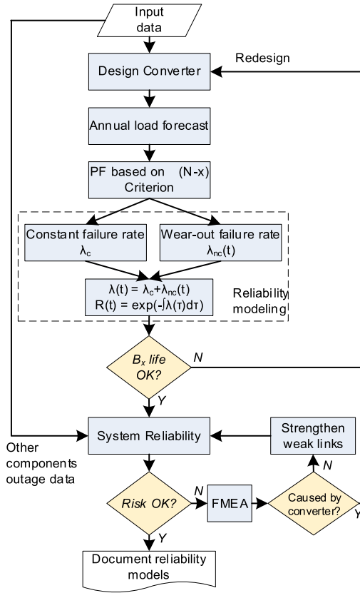
FIGURE 3. System-level design for reliability in PEPSS with N-x criteria – PF: power flow, FMEA: failure mode, and effect analysis.
