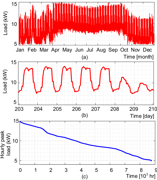
FIGURE 8. Load profile for a small clinic; (a) annual load profile, (b) daily load profile for one week, and (c) load duration curve based on hourly peak load.
