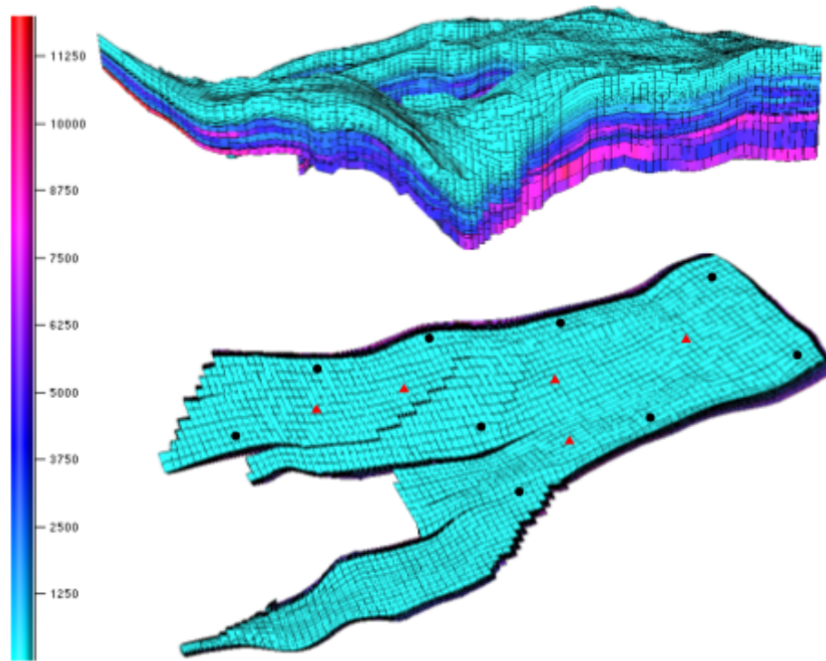
Figure 4.2: Horizontal permeability field (in md) of realization number 1 and the top view of the well locations. Black circles show the injectors and red triangles show the producers.
