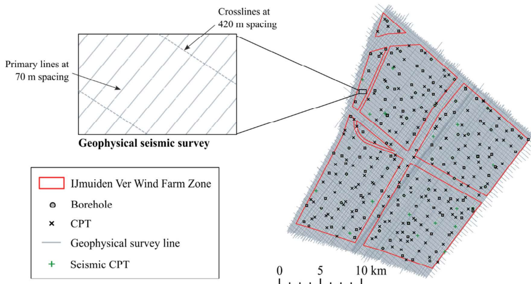
Figure 2: Site investigation data collected at IJmuiden Ver ( offshorewind.rvo.nl )
