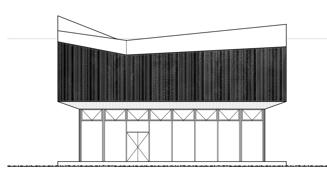
NORTH ELEVATION 1:200
