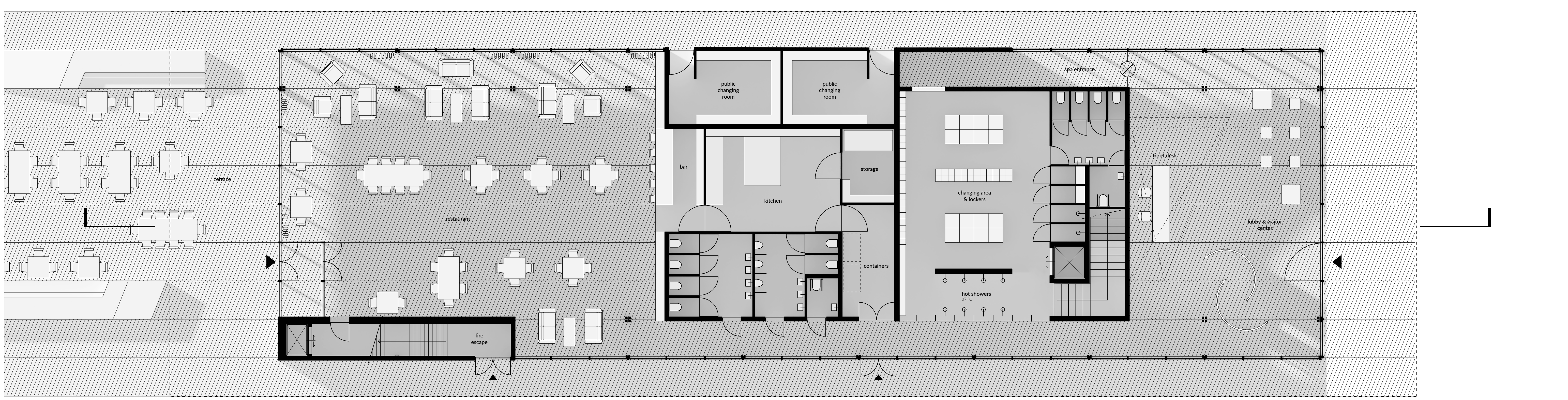
GROUND FLOOR 1:100
