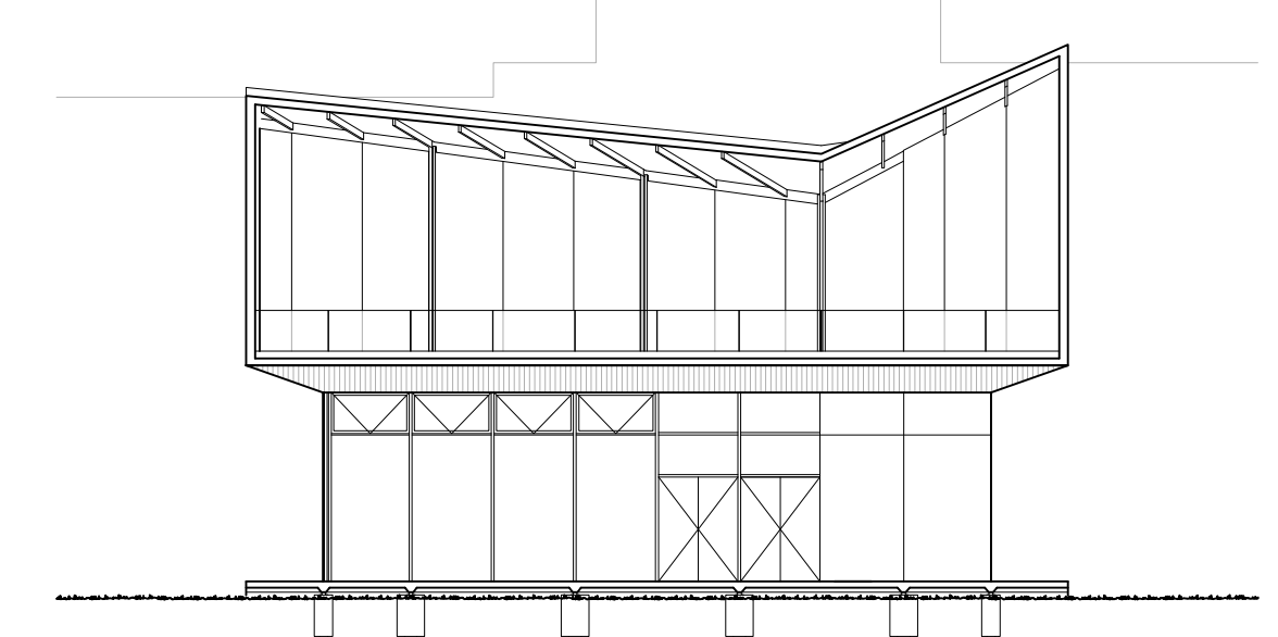
SOUTH ELEVATION 1:200
