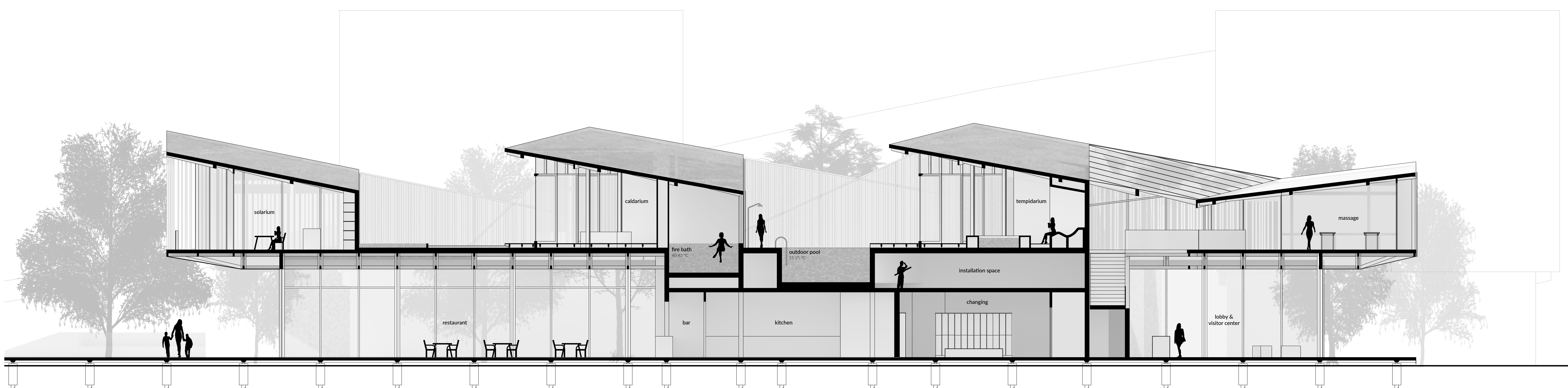
CROSS SECTION longitudinal W-E 1:100
