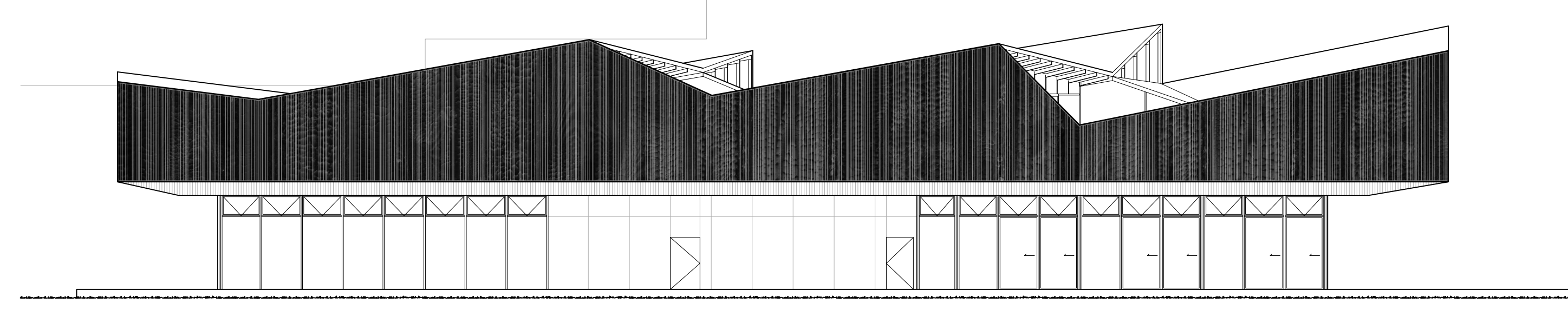
WEST ELEVATION 1:200
