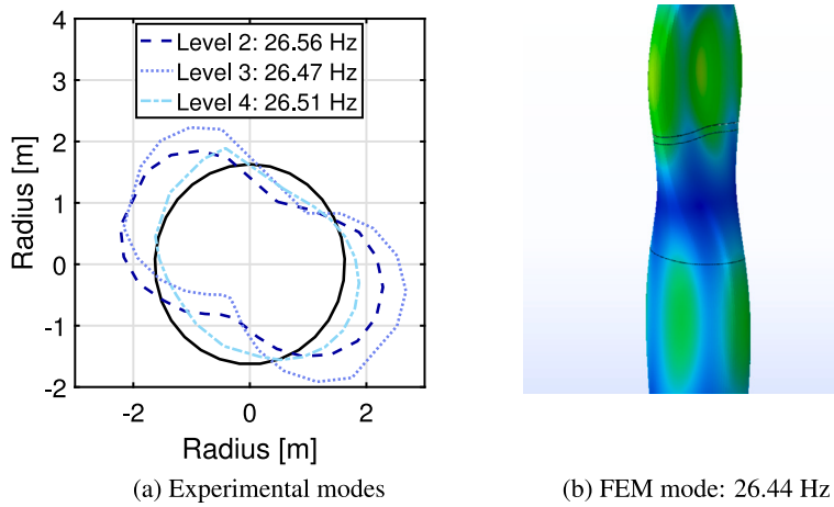
Fig. 8. Comparison between experimental and FEM mode shapes for the resonance peak around 26.5 Hz.
