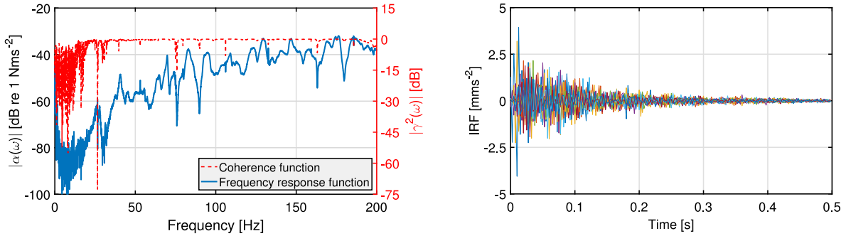
(a) Transfer function (blue line) and coherence function (red dashed line) between the measured input the dynamic response referred to sensor nr.1.
