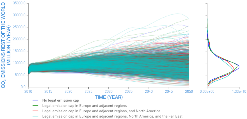
FIGURE 12: CO 2 -EMISSIONS IN THE REST OF THE WORLD (MILLION TONS PER YEAR)
