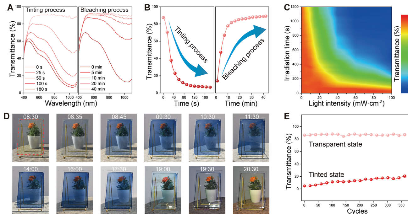
Figure 2. Photochromic effect of PC films. A) Transmittance spectra of the Cu-W-PC films prepared by the mold method during the tinting (irradiation with UV light of 365 nm, 5 mW cm -2 ) and bleaching process. The transmittance of Cu-W-PC film gradually decreased under UV light, and then the value increased and recovered after turning off the UV-light. B) Transmittance changes of the Cu-W-PC films at 1050 nm during the tinting (left) and bleaching process (right). T_{1050\text{nm}} was reduced from 90% to 9% in \approx 100 s of irradiation and recovered to a large extent ( T_{1050\text{nm}} = 85\% ) in as fast as 20 min in room light, and the value recovered completely to its original state in \approx 40 min. C) 2D mapping of the transmittance at 1050 nm of the Cu-W-PC films during the tinting process at varying solar radiation intensity/time, which shows various intermediate tinted states, indicates it is suitable to follow variable sunlight intensities during a day. D) Photographs of the Cu-W-PC films placed outside on a sunny day. E) Transmittance changes of the Cu-W-PC films at 1050 nm during more than 360 cycles of tinting and bleaching.
