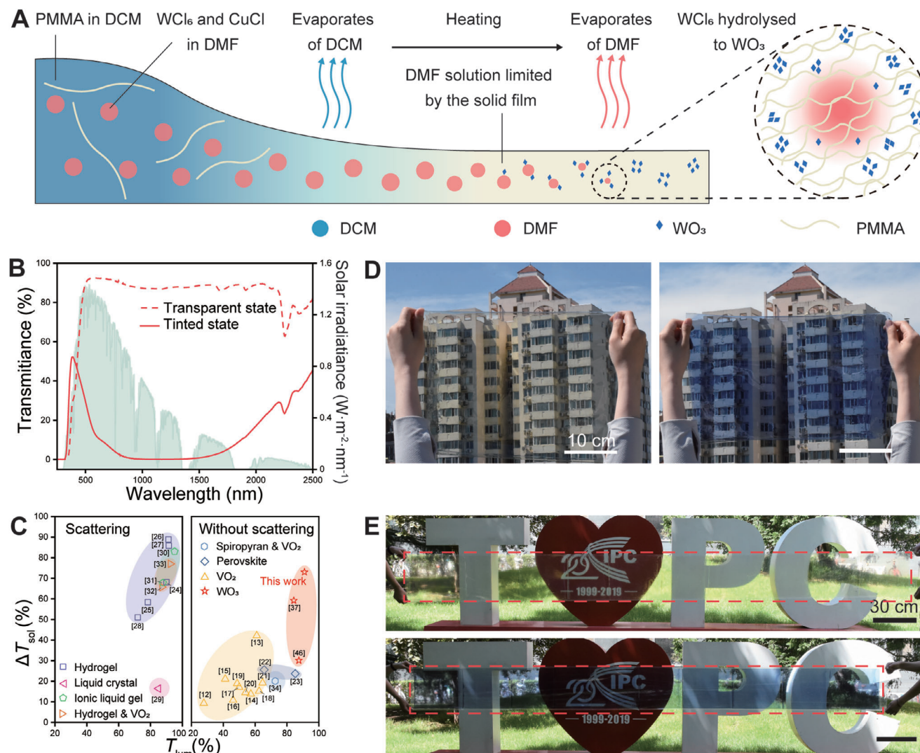
Figure 1. Preparation and working principle of PC film. A) Schematic depiction of the fabrication process for the Cu-W-PC film. The \text{WCl}_6 /DMF solution and the PMMA/DCM solution were thoroughly mixed and dried in the mold, where the PMMA and Cu-doped \text{WO}_3 , during which the PMMA and the Cu-doped \text{WO}_3 precipitated in steps. B) Transmittance spectra of the Cu-W-PC films at transparent and tinted state (by irradiation with outdoor sunlight for 6 h) against a normalized AM1.5 global solar spectrum (green shadow). C) Summary of T_{\text{lum}} and \Delta T_{\text{sol}} for passively modulated smart windows, which was divided into two types based on the presence or absence of scattering effect. The first type includes hydrogel, ionic liquid gel, and liquid crystal, which has scattering effect and affects the field of view in the tinted state. The second type includes \text{VO}_2 , perovskite and \text{WO}_3 which do not have scattering and has no effect on the field of view. The as-prepared Cu-W-PC film which has superior performance in the second type materials with the highest T_{\text{lum}} and \Delta T_{\text{sol}} . D) Photos of a 30 \times 40 \text{ cm}^2 Cu-W-PC films prepared by the blade-coating method in transparent state (left) and tinted state (right). E) Photos of a 30 \times 350 \text{ cm}^2 Cu-W-PC films on a PET substrate prepared by the blade-coating method in transparent state (top) and tinted state (bottom).
