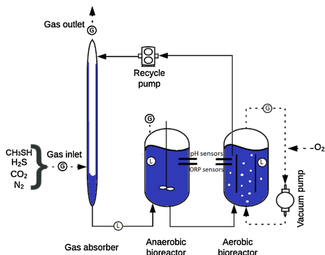
Fig. 1. Schematic representation of the experimental setup used for the experiments. G = gas sampling point, L = liquid sampling point, \text{CH}_3\text{SH} = methanethiol (MT). The blue area indicates liquid. (For interpretation of the references to colour in this figure legend, the reader is referred to the web version of this article.)
