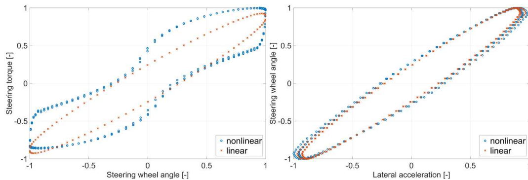
Figure 3. The characteristics of the steering system models
