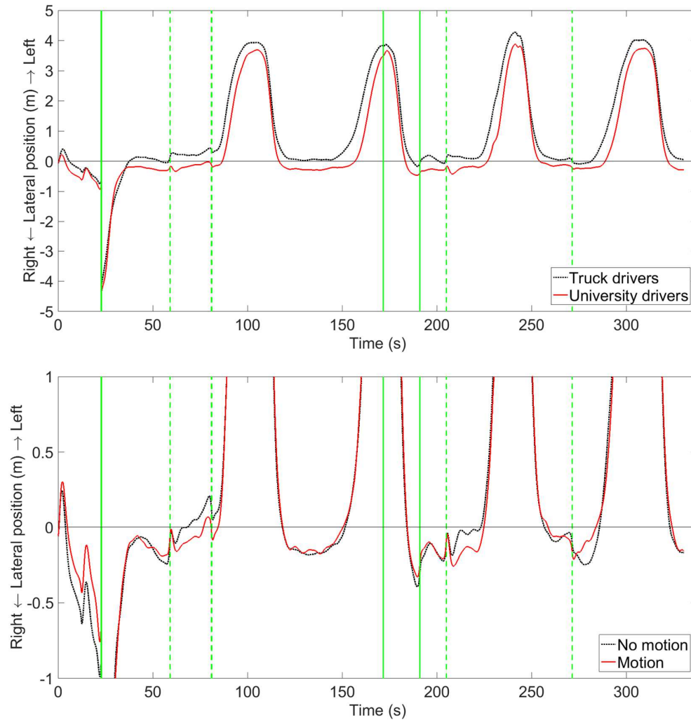
Figure 6. Mean lateral position across participants as a function of time in the session. Top = effect of participant group. Bottom = effect of motion. The jump in lateral position around 23 s is due to merging on a different driving lane. The solid vertical lines delineate right-hand curves, whereas dashed vertical lines delineate left-hand curves.
