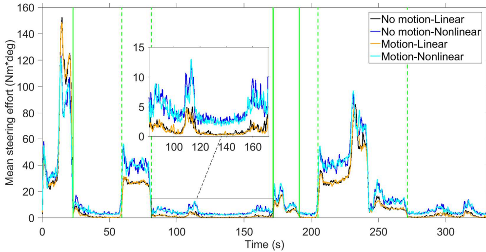
Figure 5. Mean absolute steering effort across participants as a function of time in the session. The solid vertical lines delineate right-hand curves, whereas dashed vertical lines delineate left-hand curves.
