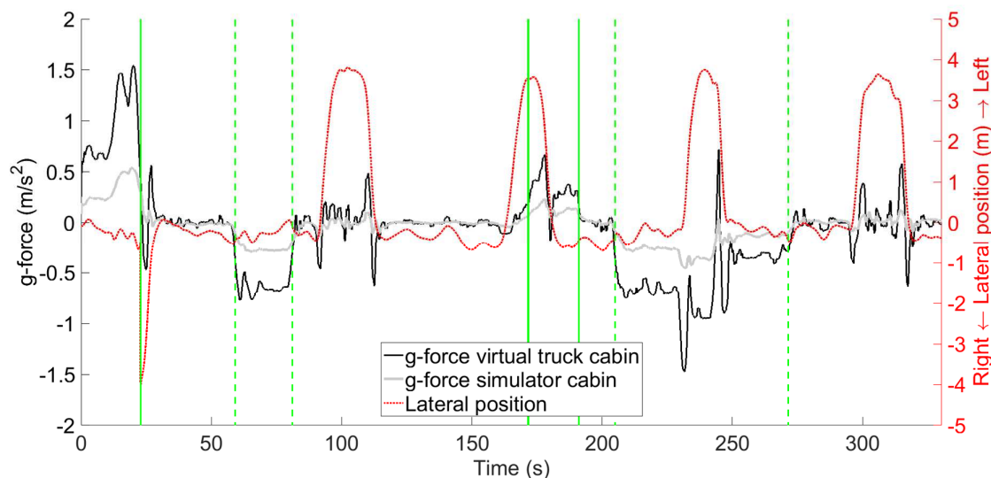
Figure 2. Lateral g-force of the virtual truck cabin, lateral g-force of the simulator cabin, and lateral position on the truck on the road for one session with motion turned on. The solid vertical lines delineate right-hand curves, whereas dashed vertical lines delineate left-hand curves. The lateral position trace shows that there were four overtaking manoeuvres in the session. The jump in lateral position around 20 s is due to merging on a different driving lane.
