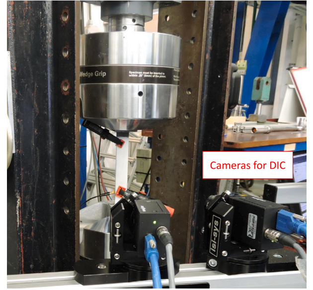
Fig. 4. A pair of 5 Megapixel cameras with 23 mm lens and 75 frames-per-second used for full-field displacements and strain measurements.
