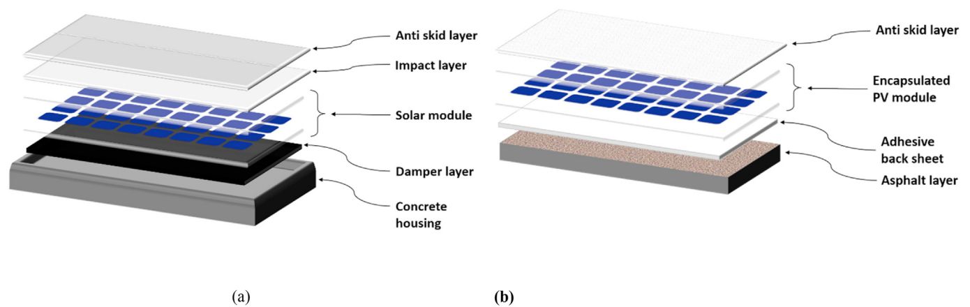
Fig. 3. Sketches (a) of a TNO Solaroad section and (b) of the solar road module concept applied in this project, inspired by the Wattway solar road technology.
