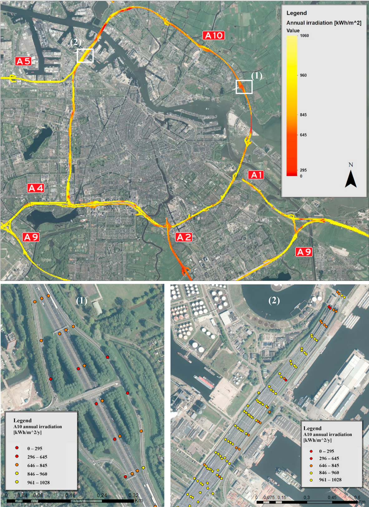
Fig. 11. Irradiation potential map of the Amsterdam ring road A10 with main injecting highways. The map helps to recognize the location where building solar roads is not advised, and also to individuate optimal installation sites.
