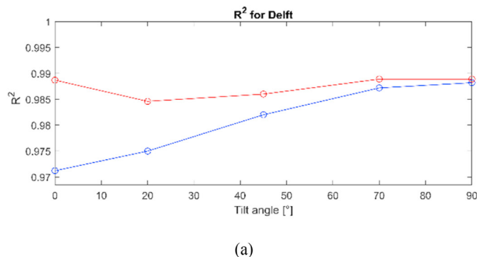
Fig. 6. Improvement of accuracy in the model with implementation of the AM correction factor: the blue line shows the accuracy of the original model expressed with R^2 versus module tilt angle. The red line represents the accuracy of the improved model after the implementation of the AM correction factor. Examples for (a) Delft (the Netherlands) and (b) Antofagasta (Chile).
