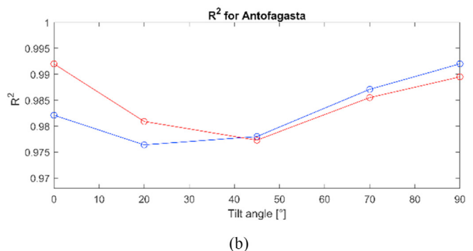
Fig. 6. Improvement of accuracy in the model with implementation of the AM correction factor: the blue line shows the accuracy of the original model expressed with R^2 versus module tilt angle. The red line represents the accuracy of the improved model after the implementation of the AM correction factor. Examples for (a) Delft (the Netherlands) and (b) Antofagasta (Chile).
