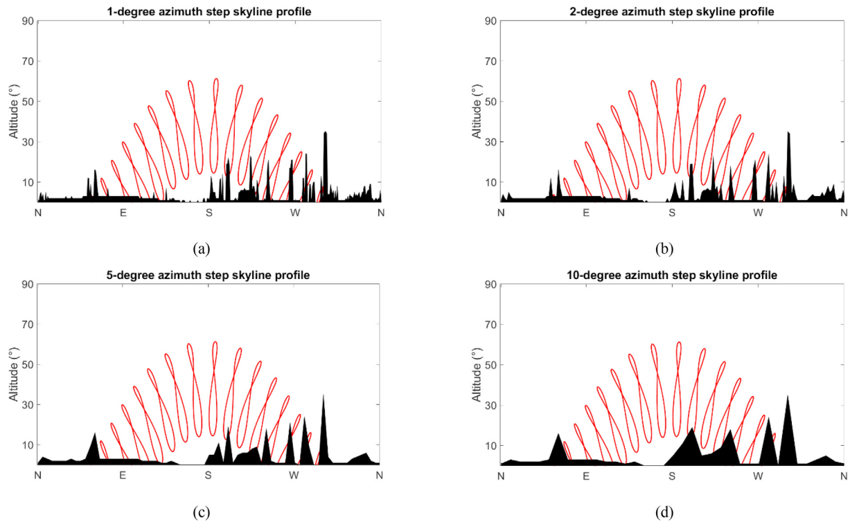
Fig. 8. Examples of how the skyline profile changes by tuning the azimuth step angle from the reference case (a) 1^\circ to (b) 2^\circ , (c) 5^\circ and (d) 10^\circ .
