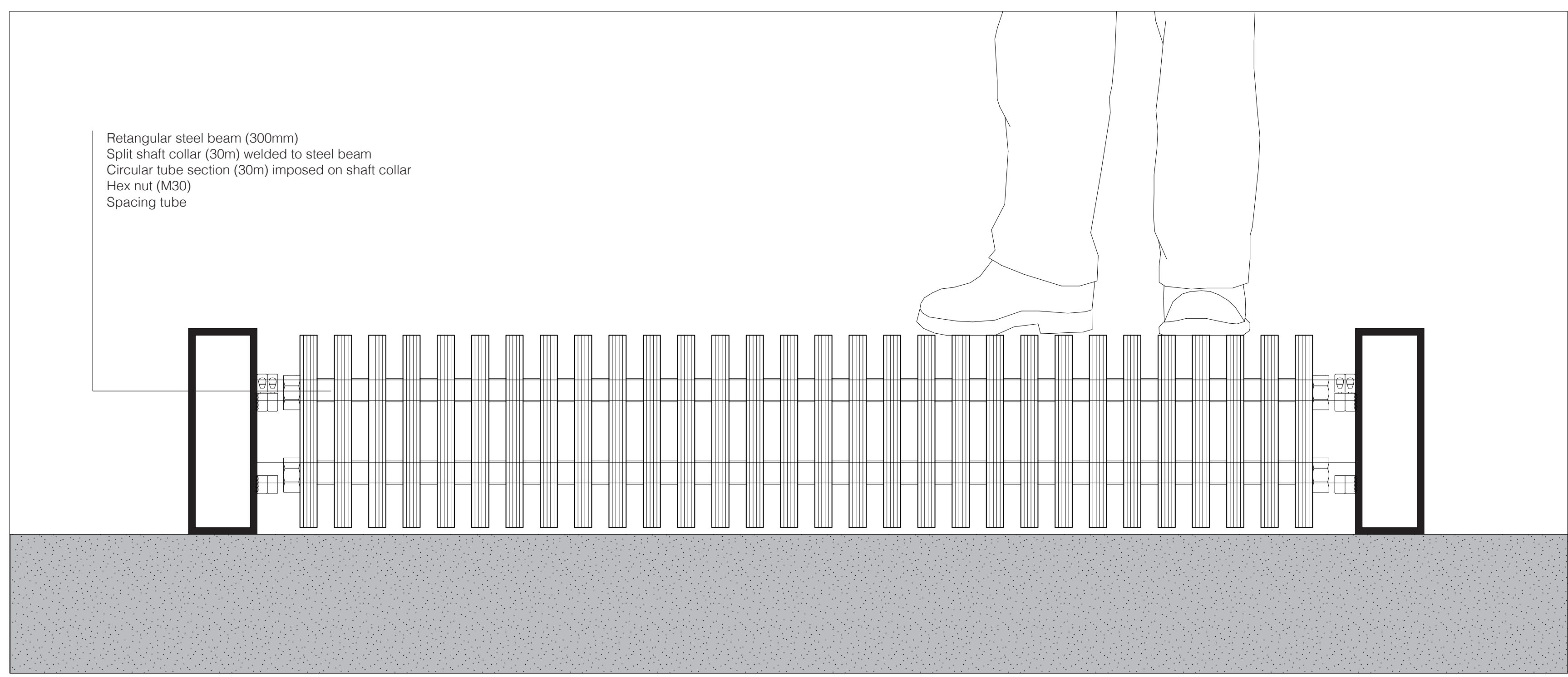
Detail 1:5 // WOODEN FLOORING ATTACHED TO STEEL BEAMS
