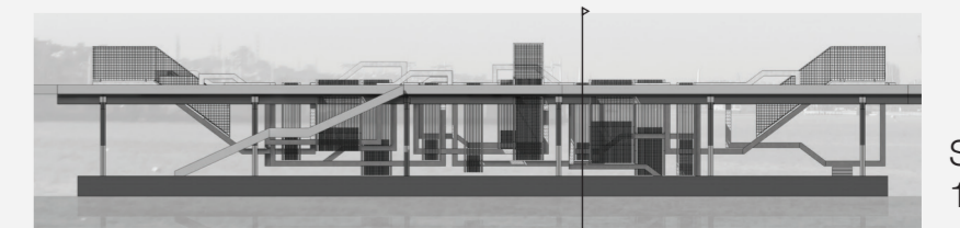
SECTION CC' 1:50
