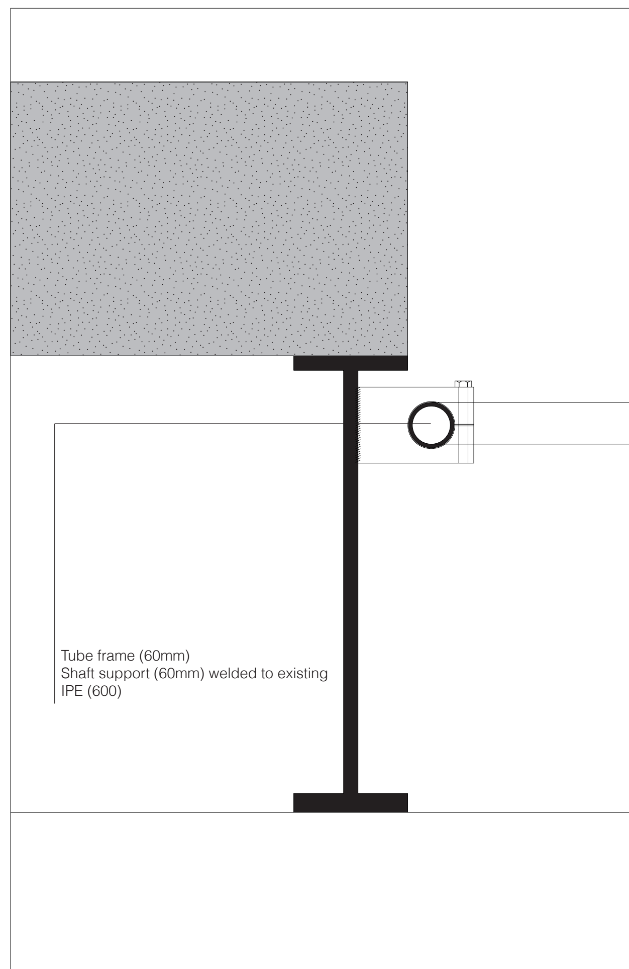
Detail 1:5 // NET FRAME CONNECTED TO EXISTING I-BEAM
