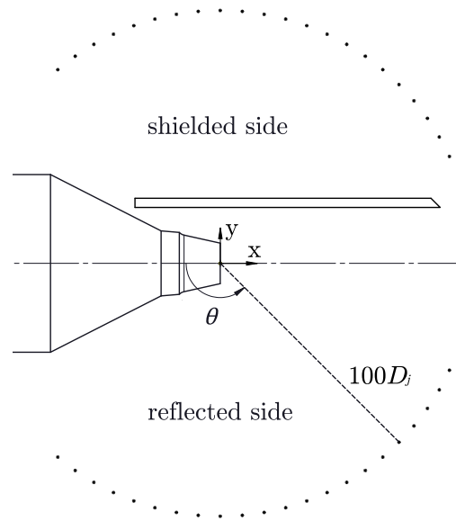
Fig. 5. Far-field microphone positions in a polar arc array, placed at the reflected and shielded sides of the jet. Microphone distance not to scale.
