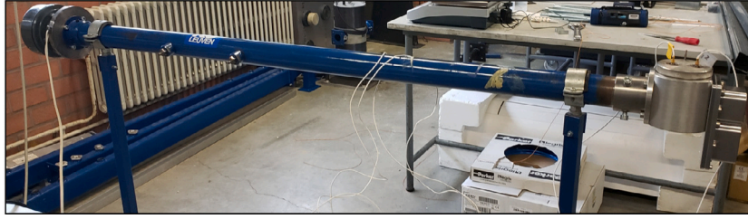
Fig. 1. Impedance tube set-up. On the left hand side of the duct there is the sound source, whereas on the right hand side there are the pressure sensors and the resonator model.
