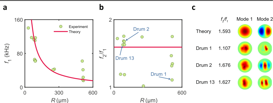
Fig. 1 | Comparison of experimental results with uniform pre-tension.
