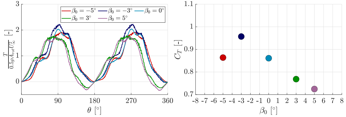
Figure 10. Experimental non-dimensional thrust of the turbine ( T ) over one turbine revolution (left-side) and corresponding thrust coefficient ( C_T ) (right-side) for different constant pitch: -5^\circ , -3^\circ , 0^\circ , 3^\circ and 5^\circ ( \beta = \beta_0 ).
