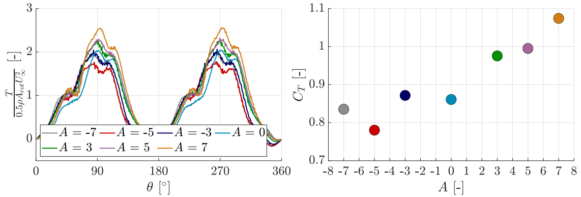
Figure 11. Experimental non-dimensional thrust of the turbine ( T ) over one turbine revolution (left-side) and corresponding thrust coefficient ( C_T ) (right-side) for different sinusoidal pitch schedules: \beta = A \sin(\theta) with A = -7 , A = -5 , A = -3 , A = 0 , A = 3 , A = 5 , A = 7 .
