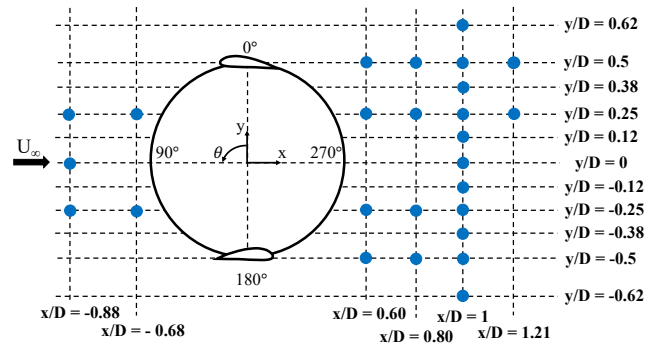
Figure 4. Hotwire measurement grid. The measurement points are coloured in blue. The coordinate system for the turbine is shown in the center.
