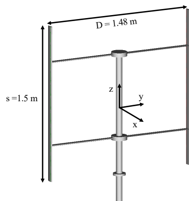
Figure 1. PitchVAWT geometry and dimensions.
