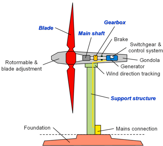
Fig. 3. Structural block of a typical HAWT system.
