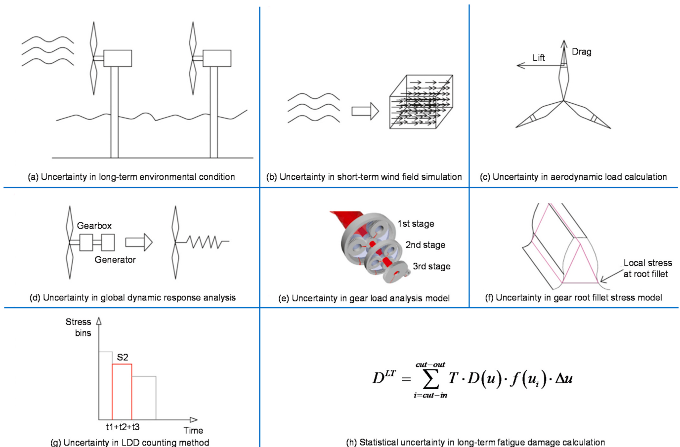
Fig. 11. Illustration of the load effect uncertainties [114].
