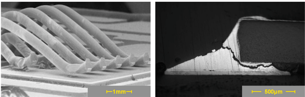
(a) wire bond lift off [148] (b) solder joint cracking [149]
