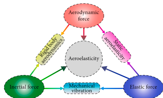
Fig. 7. Collar's triangle: interaction of different forces [66].
