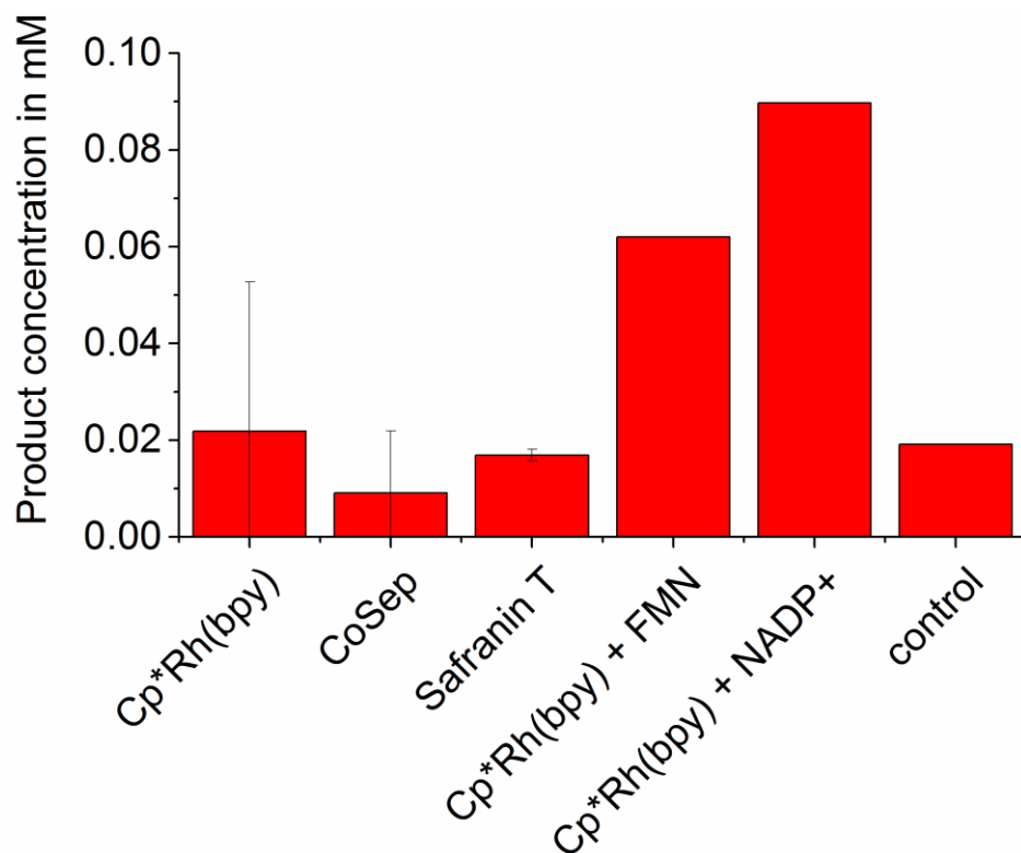
Figure 1: Product formation of dihydrocarvone at different reactions for a mediated cofactor substitution or regeneration (reaction conditions: 5 mM R(-)\text{-}
