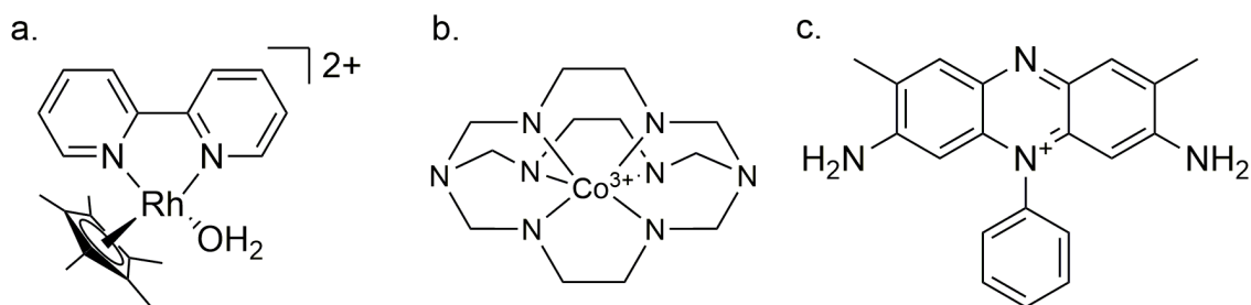
Scheme 2: Structures of the used mediators (a: [\text{Cp}^*\text{Rh}(\text{bpy})\text{Cl}]\text{Cl} ; b: cobalt sepulchrate, c. Safranin T)
