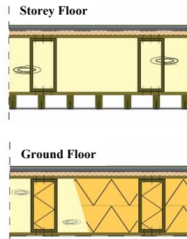
FIG. 5.2 Detailed composition of main building elements under the timber design
