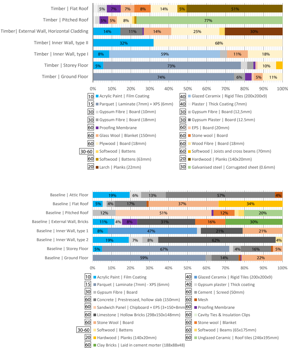
FIG. 5.10 Material impact per building component in the main building elements of the Medium House scenario in the timber and baseline construction variations. Numbers in squares are the estimated service life of the elements within each component.
