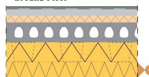
FIG. 5.3 Detailed composition of main building elements under the baseline design
