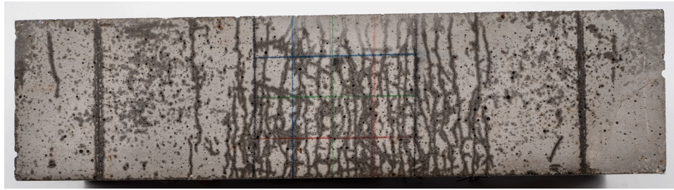
Fig. 10. Multiple micro-cracking formations in flexural harding stage (micro-cracks revealed by alcohol sprayed on the surface).
