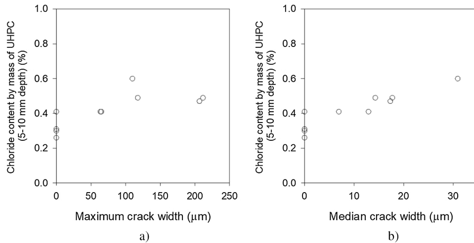
Fig. 16. Relationship between chloride content (5–10 mm depth) on a) maximum crack width and b) median crack width.
