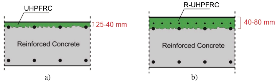
Fig. 17. Configuration of composite structural elements combining R-UHPFRC and conventional RC: a) UHPFRC layer (thickness 25–40 mm) has a protective function only; b) R-UHPFRC layer (thickness of 40–80 mm or more) has both structural resistance and protective features [57].
