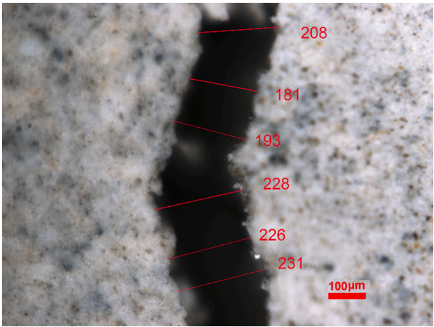
Fig. 5. Typical photo made from the measurement of one crack width (specimen “3.0%-400-5”, localisation in the matrix: A-4).
