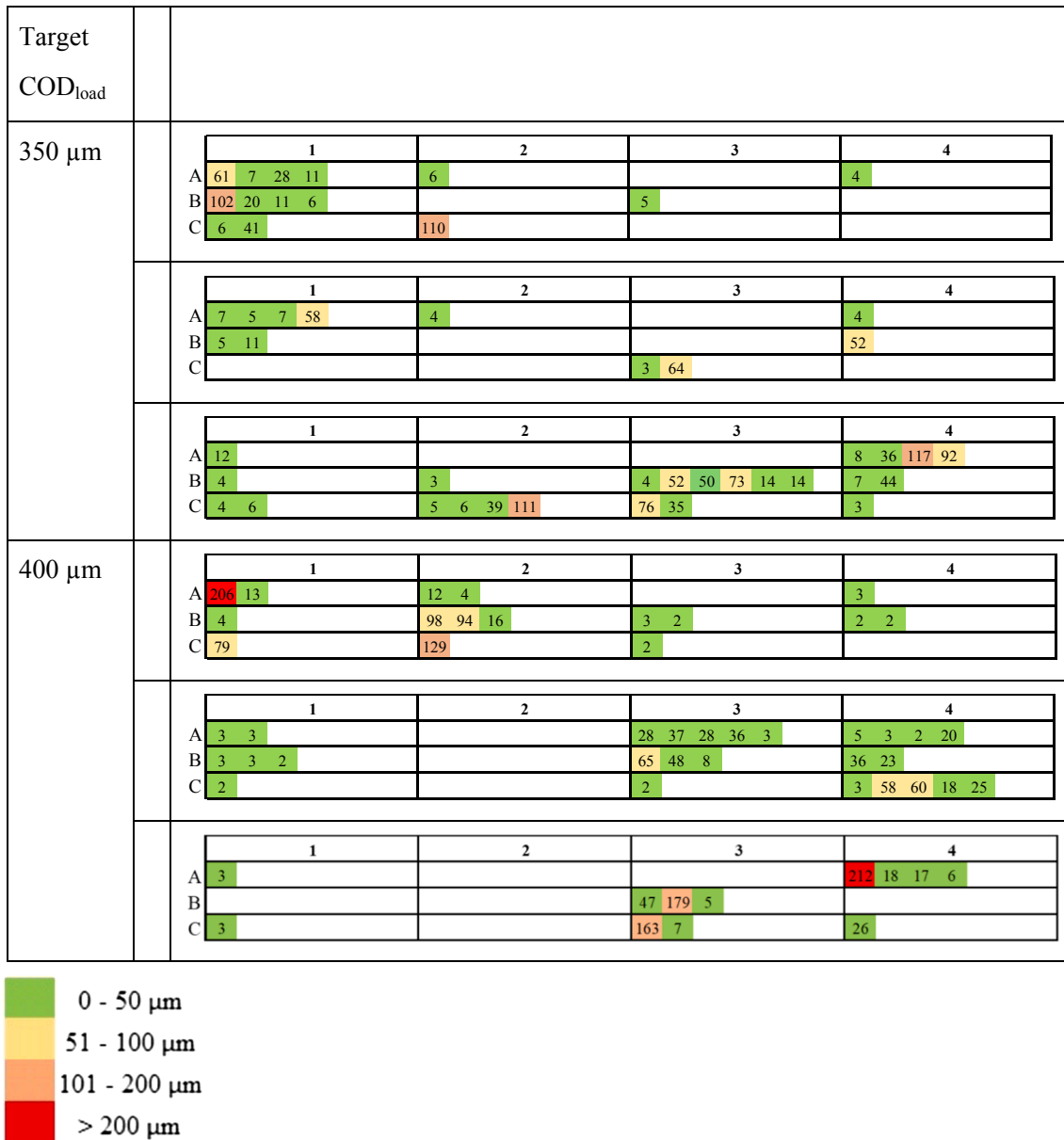
Fig. 18. Localisation of cracks observed in UHPFRC specimens and corresponding crack widths (in µm).
