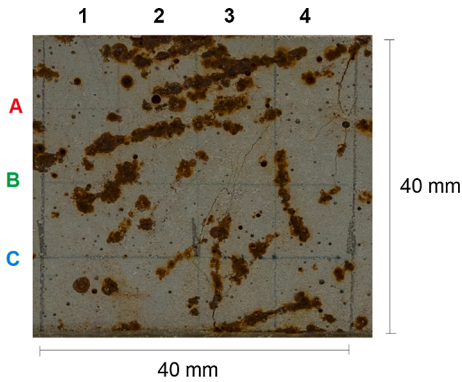
Fig. 4. Schematic matrix for crack opening measurement, the specimen “3.0%-400-5”.
