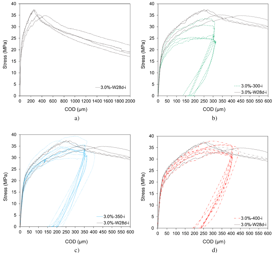
Fig. 7. a) Four-point bending load–displacement relationship after 28 days of wet curing and Load–displacement curves obtained at 28 days while establishing target CODs: b) COD_{load} = 300 \mu m , c) COD_{load} = 350 \mu m and d) COD_{load} = 400 \mu m .
