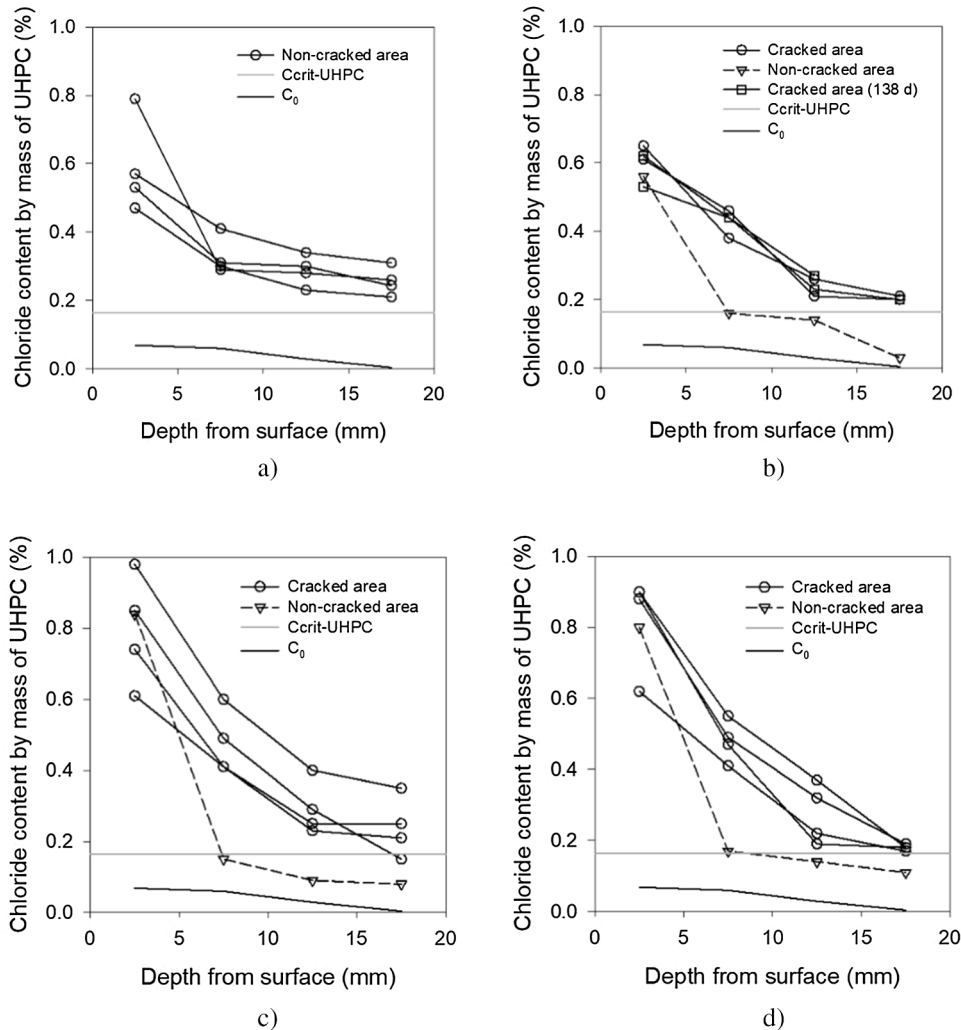
Fig. 15. Chloride profiles for UHPFRC series: a) 3.0%-0-i; b) 3.0%-300-i; c) 3.0%-350-i and d) 3.0%-400-i specimens;
