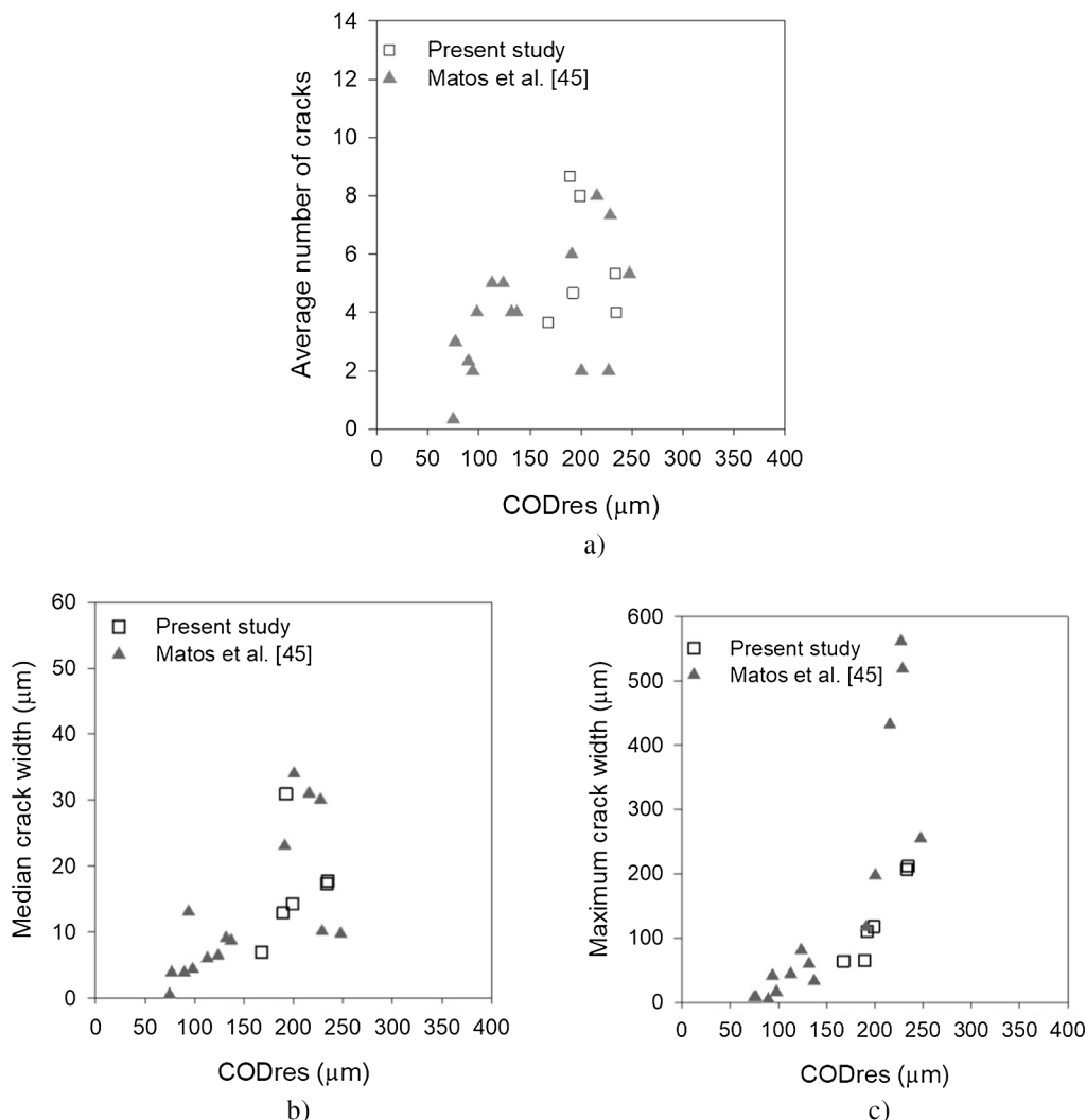
Fig. 9. Crack pattern parameters: a) Average number of cracks over 40 mm; b) Median crack width; c) Maximum crack width.
