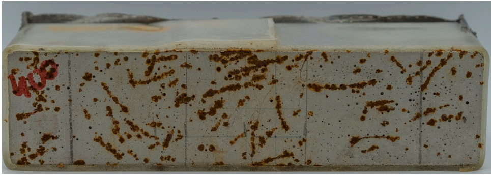
Fig. 3. Tensile surface of specimen “3.0%-400-5” after cracking.
