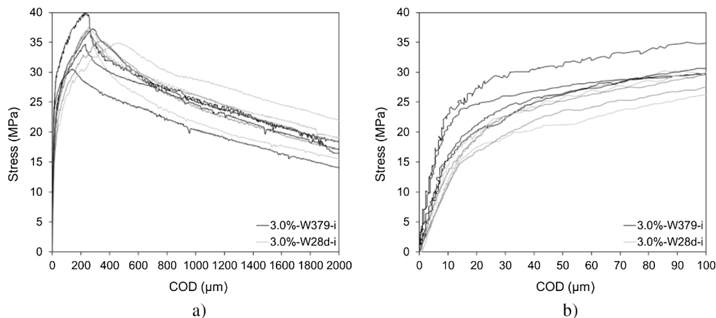
Fig. 12. a) Four-point bending load-displacement relationships for 28 and 379 old days up to softening area and b) Load-displacement curves zoom up to COD = 100 \mu m .
