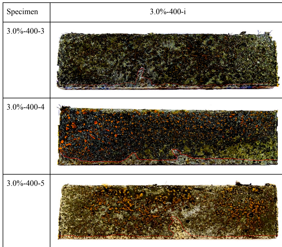
Fig. 21. Chlorides ingress of 3.0%-400-i specimens (penetration depth of chloride ions in lighter part).
