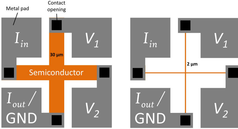
Figure 5.4: Greek-cross resistors used in this work with resistor beam widths of 30 and 2 \mu\text{m} .
