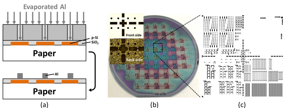
Figure 6.6: Masking process schematic for metal patterns (a), optical image of the mask with comparisons of front to backside (b), and the design of a single die (c).
