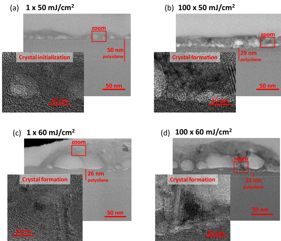
Figure 3.14: Cross-sectional TEM images of polysilane exposed to a KrF laser with different treatments: 1x 50 mJ/cm 2 (a), 100x 50 mJ/cm 2 (b), 1x 60 mJ/cm 2 (c), and 100x 60 mJ/cm 2 (d).
