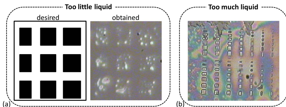
Figure 7.6: Effect of stamping with too little (a) and too much (b) liquid.
