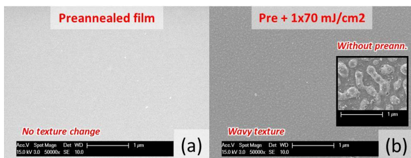
Figure A.1: SEM images of a excimer pre-annealed film (a), and a pre-annealed film with a subsequent exposure to 1 pulse of 70 \text{ mJ/cm}^2 (b).
