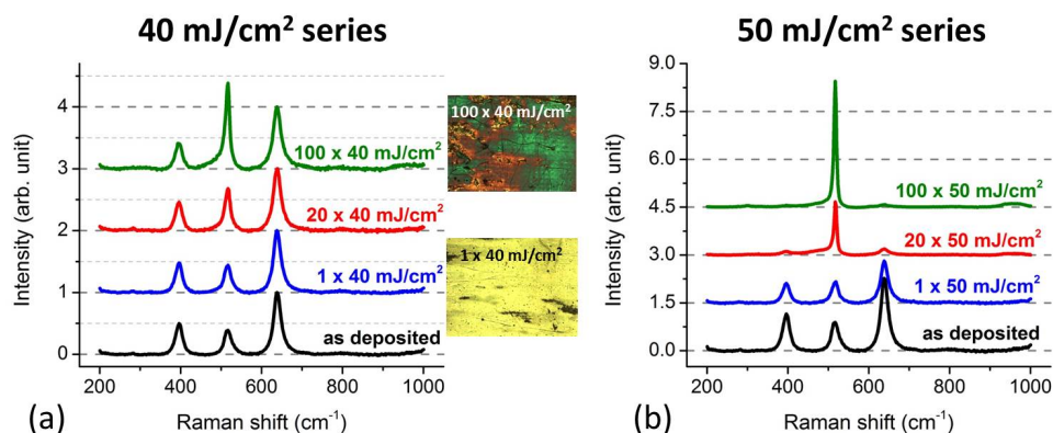
Figure 6.4: Raman spectra of polysilane annealed with multiple pulse excimer laser energy densities of 40 mJ/cm 2 (a), and 50 mJ/cm 2 (b).
