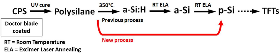
Figure 2.11: Proposed process flow of the direct transformation from polysilane to poly-Si.
