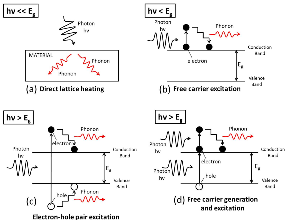
Figure 4.1: Illustrations of laser energy absorption mechanisms for photon energy h\nu \ll bandgap energy E_g (a), h\nu < E_g (b), h\nu > E_g (c), and h\nu > E_g with high intensity (d).
