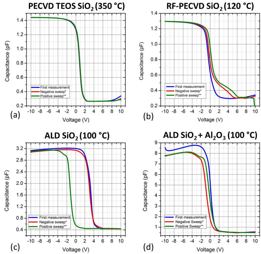
Figure 5.3: Capacitance to voltage measurements for four different types of oxides: PECVD TEOS SiO 2 (a), RF-PECVD SiO 2 (b), ALD SiO 2 (c), ALD SiO 2 + Al 2 O 3 (d). Each displaying three curves: first measurement (blue), repeated measurements (red), and opposite voltage sweep (green).
