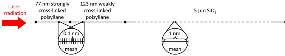
Figure 8.1: 1-Dimensional COMSOL simulation model of a polysilane on top of a glass substrate divided into a strongly and a weakly cross-linked fraction.
