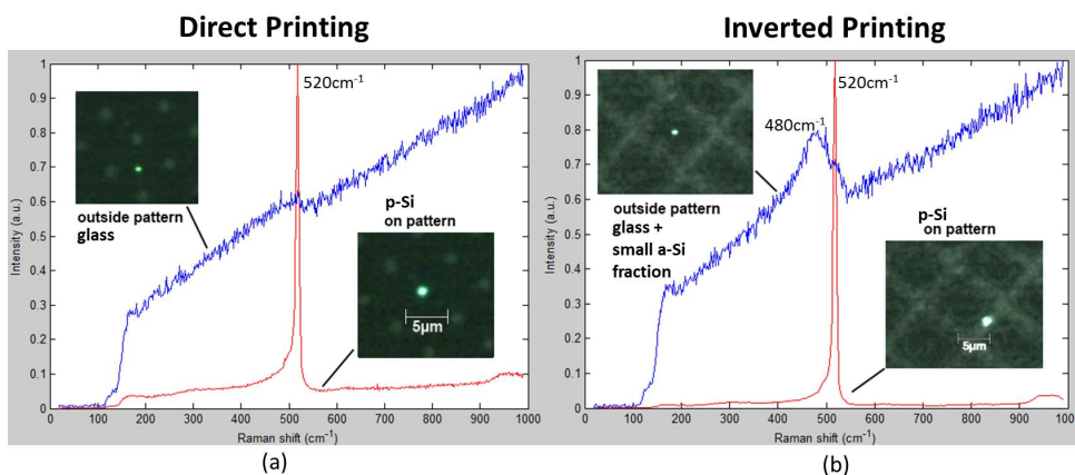
Figure 7.10: Raman spectra of stamped results showing the light pattern to be poly-Si and the dark area to have no silicon. Direct printing (a), and inverted printing (b).
