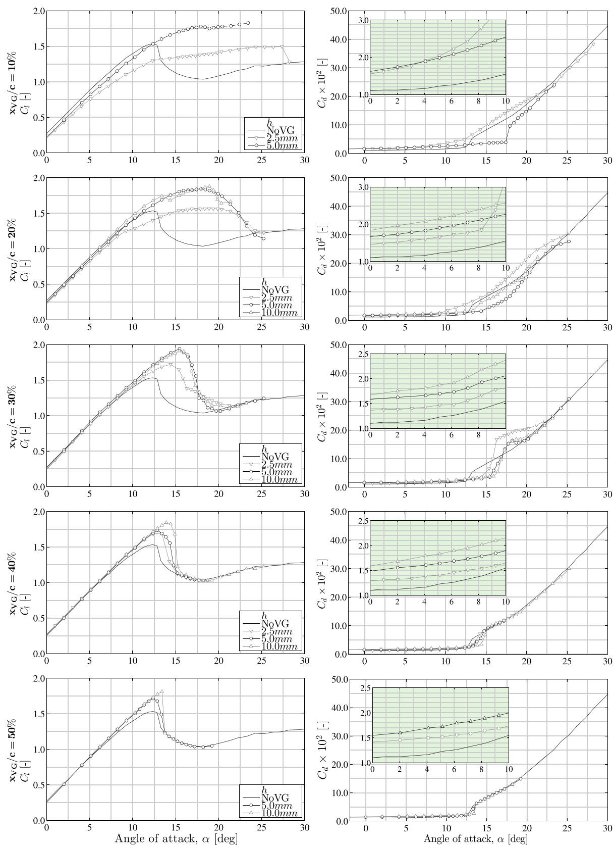
FIGURE A1 Sensitivity to array chordwise placement and vortex generator vane height. Graphs are grouped into rows according to the array chordwise placement (top-bottom): x_{VG} = 10\%c to 50\%c . NoVG, uncontrolled airfoil [Colour figure can be viewed at wileyonlinelibrary.com ]
