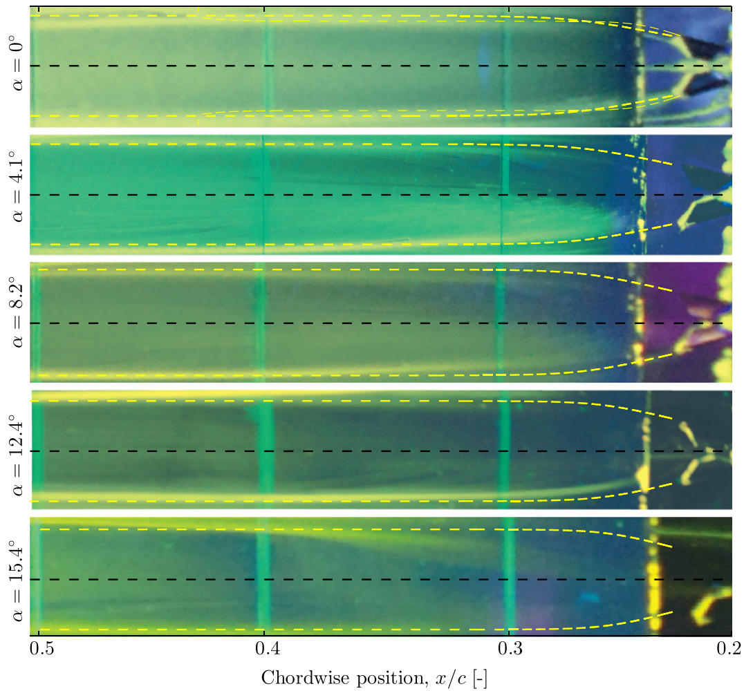
FIGURE 10 Base design near wake oil-flow visualisations for increasing angles of attack. Flow direction: right to left [Colour figure can be viewed at wileyonlinelibrary.com ]
