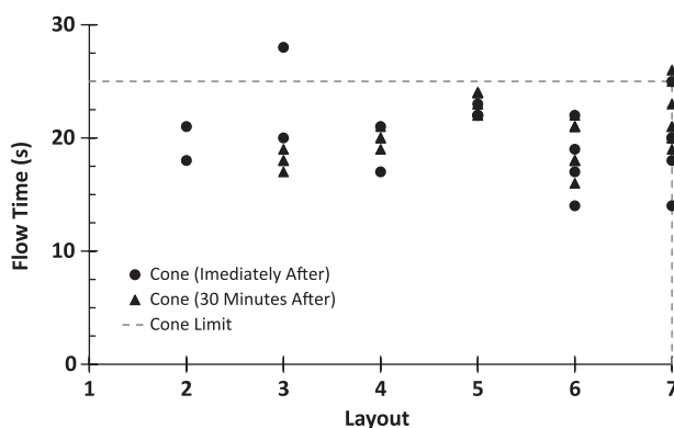
FIG. 7 Grout fluidity test results.
