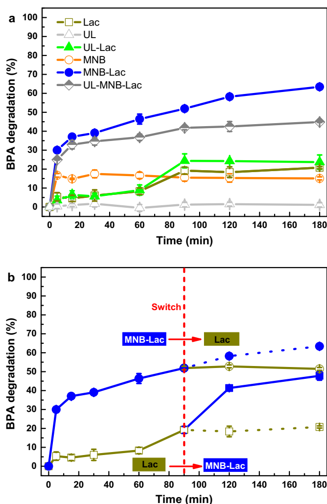
Fig. 2. a. BPA degradation by Lac, UL, UL-Lac, MNB, MNB-Lac, and UL-MNB-Lac. b. Effect of the procedural switch between Lac (90 min) and MNB-Lac (90 min) on BPA degradation. Conditions: 1.20 g \cdot L ^{-1} Lac, 1.0 mM BPA, pH 8, 30 ^{\circ} C. Shaker: 150 r \cdot min ^{-1} . UL: 60 W power, 40 kHz frequency. MNB: 30 mL \cdot min ^{-1} air intake, 1.5 m outlet pipe.
