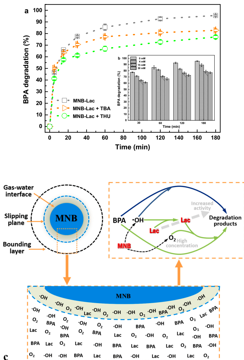
Fig. 4. a. BPA degradation with MNB-Lac contained different scavengers. Conditions: 0.60 g·L -1 Lac, 1.0 mM BPA, pH 8, 40 °C, 30 mL·min -1 air intake, 8.6 m outlet pipe, 15 mM TBA, 30 mM THU. b. BPA degradation with MNB-Lac at different THU concentrations. c. The possible mechanism of BPA degradation by MNB-Lac.
