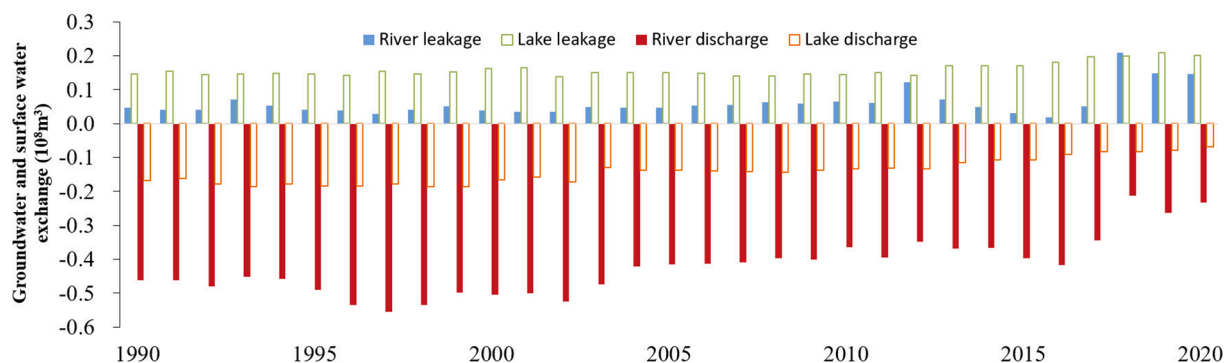
Fig. 11. Water exchange between groundwater and surface water.
