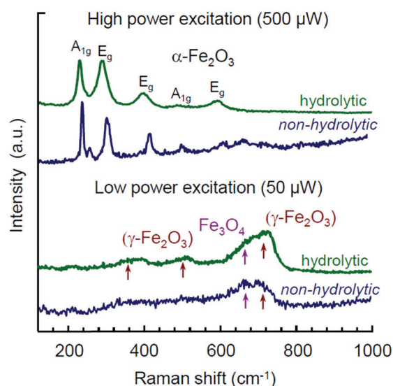
Fig. 5 Raman spectra for Mt NPs synthesized by hydrolytic and non-hydrolytic (in i -PrOH) routes measured at laser powers of 50 and 500 \mu\text{W} .
