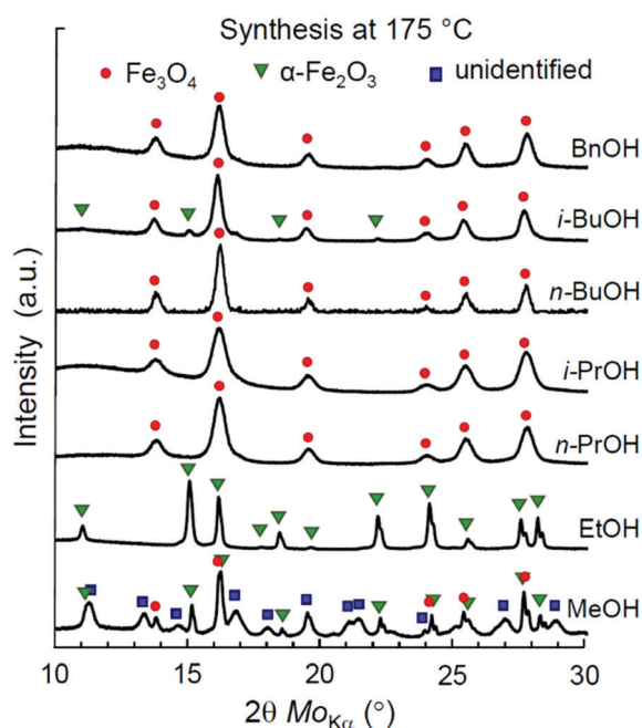
Fig. 1 XRD patterns of iron oxide nanoparticles synthesized in lower alcohols at 175 °C.
