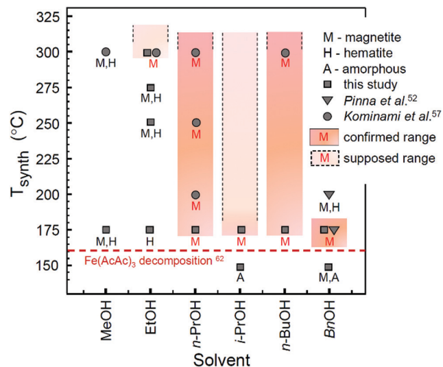
Fig. 4 Diagram of iron oxide formation in a solvothermal system of \text{Fe}(\text{AcAc})_3 and lower alcohols. Filled colour areas designate the single-phase Mt product. The plotted data are taken from this study (synthesis time: 24 h) and adopted from ref. 52 (synthesis time: 48 h) and ref. 57 (synthesis time: 2 h). The initial decomposition temperature for \text{Fe}(\text{AcAc})_3 (horizontal dashed line) is taken from ref. 62.
