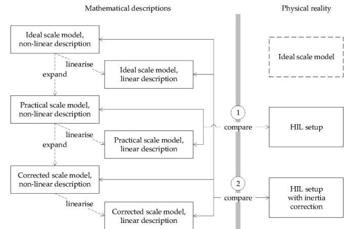
Fig. 16. Approach to validating mathematical descriptions and proposed solutions for scale effects, using numerical simulations and HIL experiments. Note that the ideal scale model has a dashed edge as it does not actually exist.
