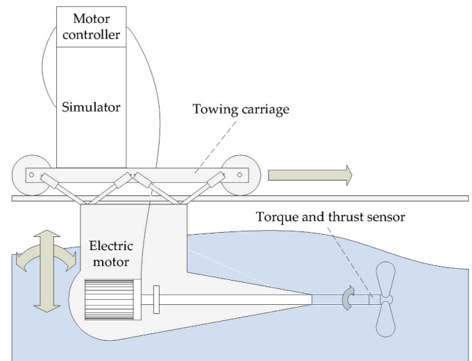
Fig. 2. Schematic drawing of the HIL open water setup, used to emulate the dynamic behaviour of the diesel-mechanical propulsion system shown in Fig. 1.
