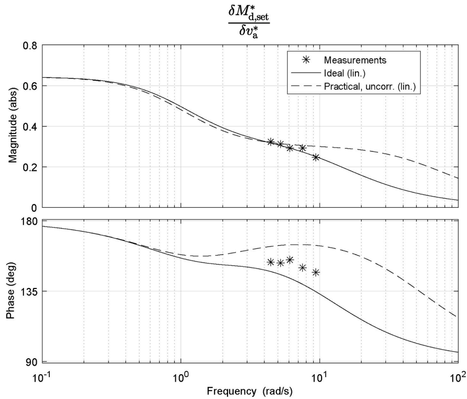
Fig. 22. Linear simulations and HIL measurements of closed loop response of simulated engine torque on waves, with numerical inertia correction. The corresponding transfer function is given in Eq. (48). This Figure is based on the data in exp_234.mat , exp_235.mat , exp_236.mat , exp_237.mat and exp_238.mat , stored in the measurement data repository (Huijgens, 2020).
