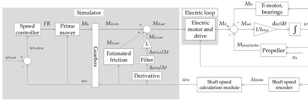
Fig. 15. Block diagram of the practical dynamic open water test with numerical inertia correction, based on measured shaft speed.
