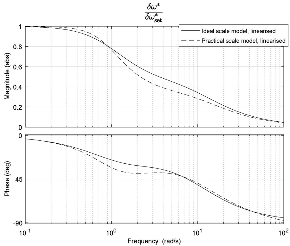
Fig. 10. Bode diagram of linearised response of shaft speed \delta\omega^* on set speed \delta\omega_{set}^* with distortions due to an improperly tuned current controller. Parameters and equilibrium values are given in Tables B.9 and B.10 ; current controller settings K_{p,i}^* and K_{p,i}^* are both set to 1 for the practical scale model.
