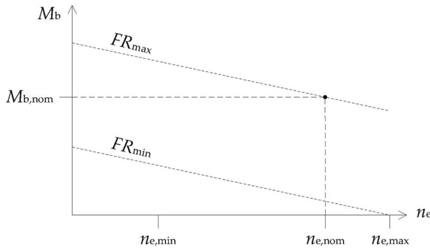
Fig. 6. Fuel rack map visualising the relation between engine speed, fuel rack setting and engine torque for the diesel engine in this paper.
