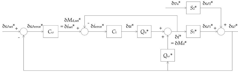
Fig. 9. Graphical representation of the linearised practical scale model or HIL setup.
