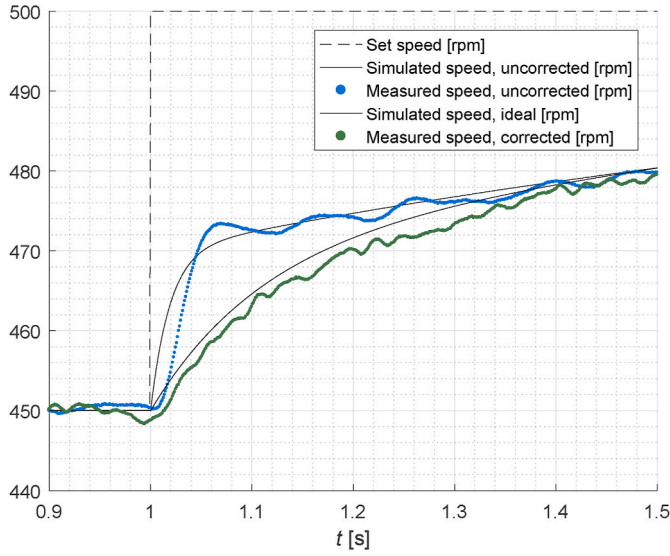
Fig. 20. Response of model scale engine speed n_e on a step change in speed setting n_{e,set} from 450 to 500 rpm (full scale equivalent speed), for the ideal, uncorrected and corrected scale models. A close-up of the first half second of response is shown for HIL measurements and non-linear simulations. This Figure is based on the data in exp_220.mat (without inertia correction) and exp_219.mat (with inertia correction), stored in the measurement data repository (Huijgens, 2020).
