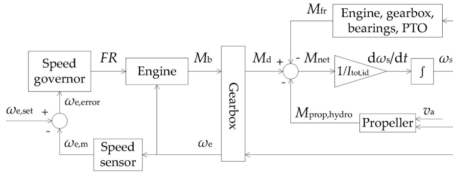
Fig. 3. Block diagram of the ideal scale model from speed setting to shaft speed. In this paper, a diesel-mechanical propulsion system is considered such as drawn in Fig. 1. The ideal scale model is the full scale propulsion system, scaled down without scale effects.
