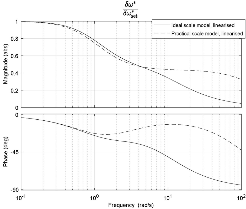
Fig. 12. Bode diagram of linearised response of shaft speed \delta\omega^* on set speed \delta\omega_{set}^* with distortions due to incorrect moment of inertia. Response is shown of the ideal scale model and a practical scale model with a moment of inertia which is 9.8% of its ideal value. Apart from the moment of inertia of the practical scale model, parameters for both scale models are given in Table B.9.
