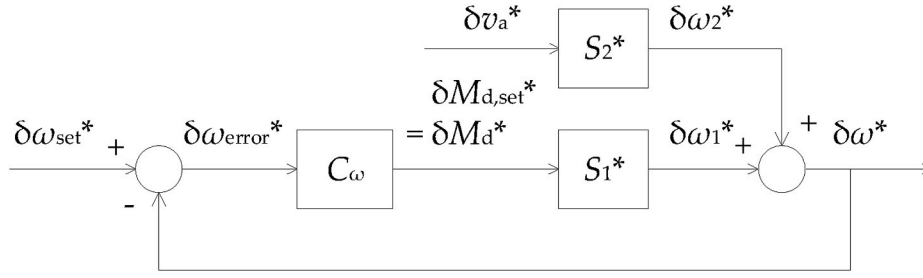
Fig. 8. Graphical representation of the linearised ideal scale model.
