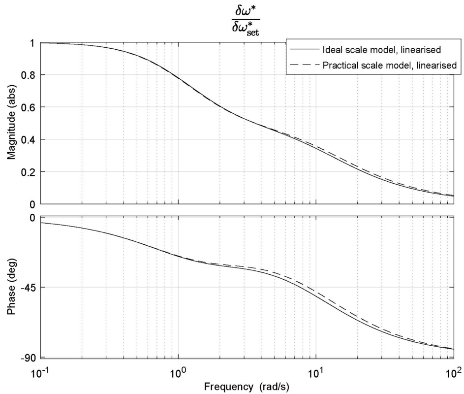
Fig. 11. Bode diagram of linearised response of shaft speed \delta\omega^* on set speed \delta\omega_{set}^* with distortions due to model scale friction. Response is shown of the ideal scale model and a practical scale model with an equilibrium torque increased by 10% relative to its ideal value. Apart from the equilibrium torque of the practical scale model, parameters for both scale models are given in Table B.9 .
