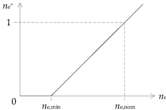
Fig. 4. Scaling of the input signal, measured shaft speed, as commonly done in shaft speed governors of marine diesel engines.
