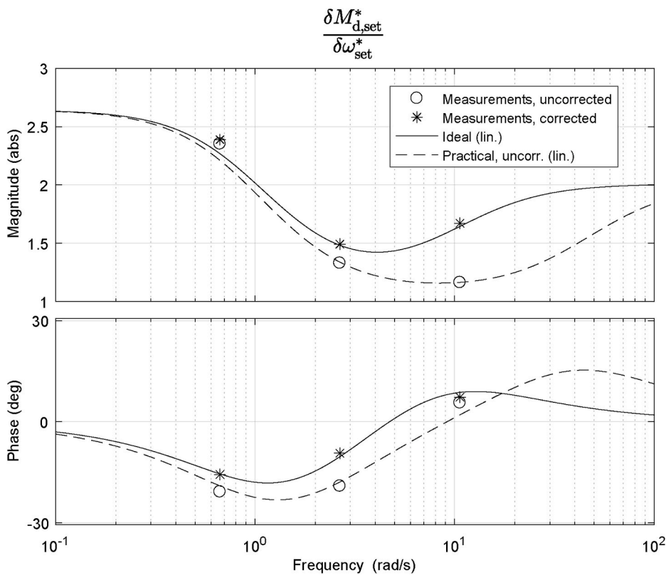
Fig. 19. Simulated and measured closed loop response of drive torque on set speed. Measurements with and without inertia correction are shown, while linear simulations are shown for the ideal scale model and practical scale model without inertia correction. The corresponding transfer function is given in Eq. (46). This Figure is based on the data in exp_216.mat , exp_217.mat , exp_218.mat (without inertia correction) and exp_212.mat , exp_213.mat , exp_214.mat (with inertia correction), stored in the measurement data repository (Huijgens, 2020).
