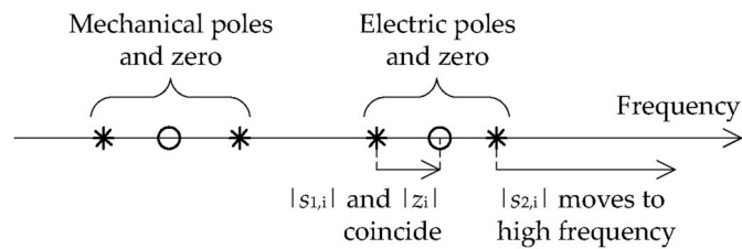
Fig. 13. To avoid dynamic distortion, the electric poles s_{1,i} and s_{2,i} and electric zero z_1 must be cancelled out and moved away from the mechanical poles and zero.
