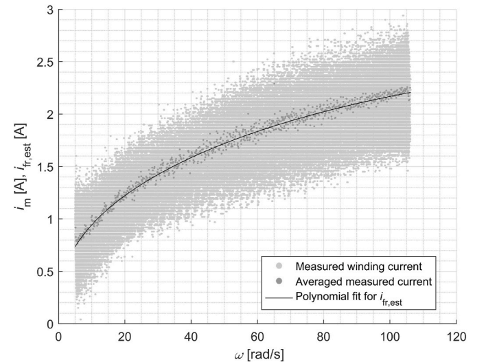
Fig. 14. Polynomial regression of measured friction current at shaft speeds between 50 and 1000 rpm. In the shown measurement run, the shaft was completely submerged, with the propeller, streamline caps and fairing dismounted. The dark gray points indicate the averaged measured current per 0.1 rad/s increment of shaft speed. The polynomial fit has an R^2 of 0.986; Table 1 shows the corresponding coefficients. This Figure is based on the data in cal_085.mat , stored in the measurement data repository (Huijgens, 2020).
