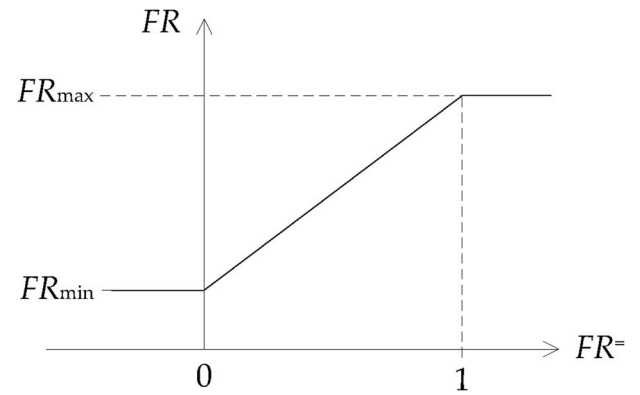
Fig. 5. Scaling of the output signal, the fuel rack setting, as commonly done in shaft speed governors of marine diesel engines.
