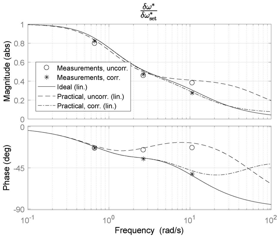
Fig. 18. Simulated and measured closed loop response of shaft speed on set speed. Measurements with and without inertia correction are shown, while linear simulations are shown for the ideal scale model, practical scale model with inertia correction and practical scale model without inertia correction. The corresponding transfer function is given in Eq. (45). This Figure is based on the data in exp_216.mat , exp_217.mat , exp_218.mat (without inertia correction) and exp_212.mat , exp_213.mat , exp_214.mat (with inertia correction), stored in the measurement data repository (Huijgens, 2020).
