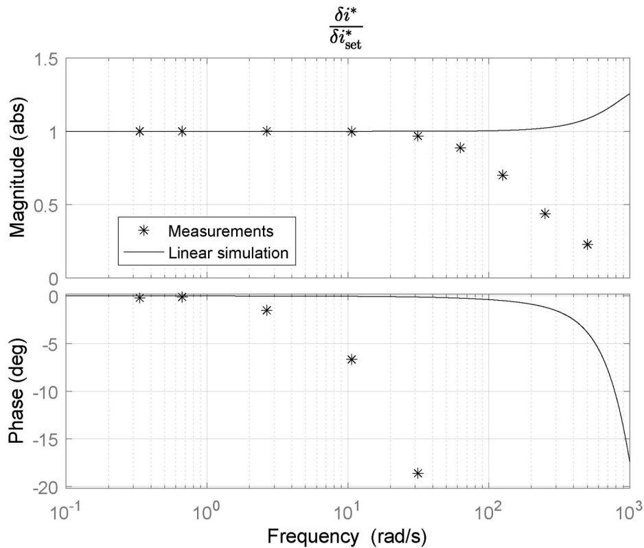
Fig. 17. Simulated and measured response of current i on current setting i_{\text{set}} . The current controller has the actual settings given in Table 2. This Figure is based on the data in exp_174.mat , exp_175.mat , exp_176.mat , exp_177.mat , exp_178.mat , exp_179.mat , exp_180.mat , exp_181.mat and exp_182.mat , stored in the measurement data repository (Huijgens, 2020).
