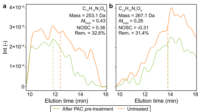
Fig. 6. EICs and AETs (dashed lines) of two molecular formulas with comparable removal, before and after PAC 40 mg L -1 pre-treatment: a, C 11 H 11 N 1 O 6 ; b, C 13 H 17 N 1 O 5 .
