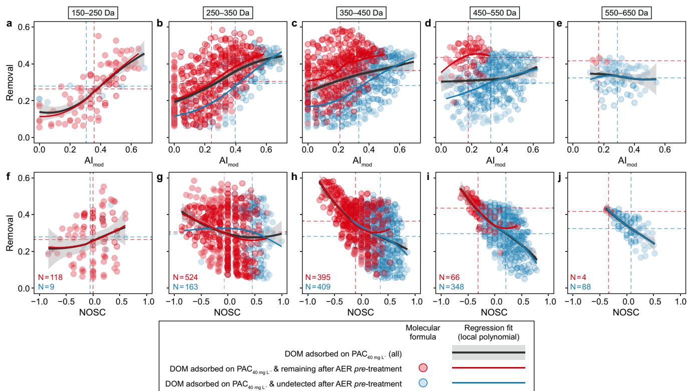
Fig. 5. Removed fraction (based on FT-ICR-MS intensities) of DOM adsorbed on PAC 40 mg L -1 and remaining (red) or undetected (blue) after AER pre-treatment plotted vs. Al_{mod} (a–e) or NOSC (f–j) for different mass ranges: 150–250 Da (a, f), 250–350 Da (b, g), 350–450 Da (c, h), 450–550 Da (d, i), and 550–650 Da (e, j). Local polynomial regression fits with 95% confidence interval, mean Al_{mod} or NOSC, and the number of molecular formulas (N) are provided. Note: the compounds undetected after PAC 40 mg L -1 pre-treatment (100% removal) and molecular formulas with peak intensity < 10 3 in untreated DOM samples are not included.
