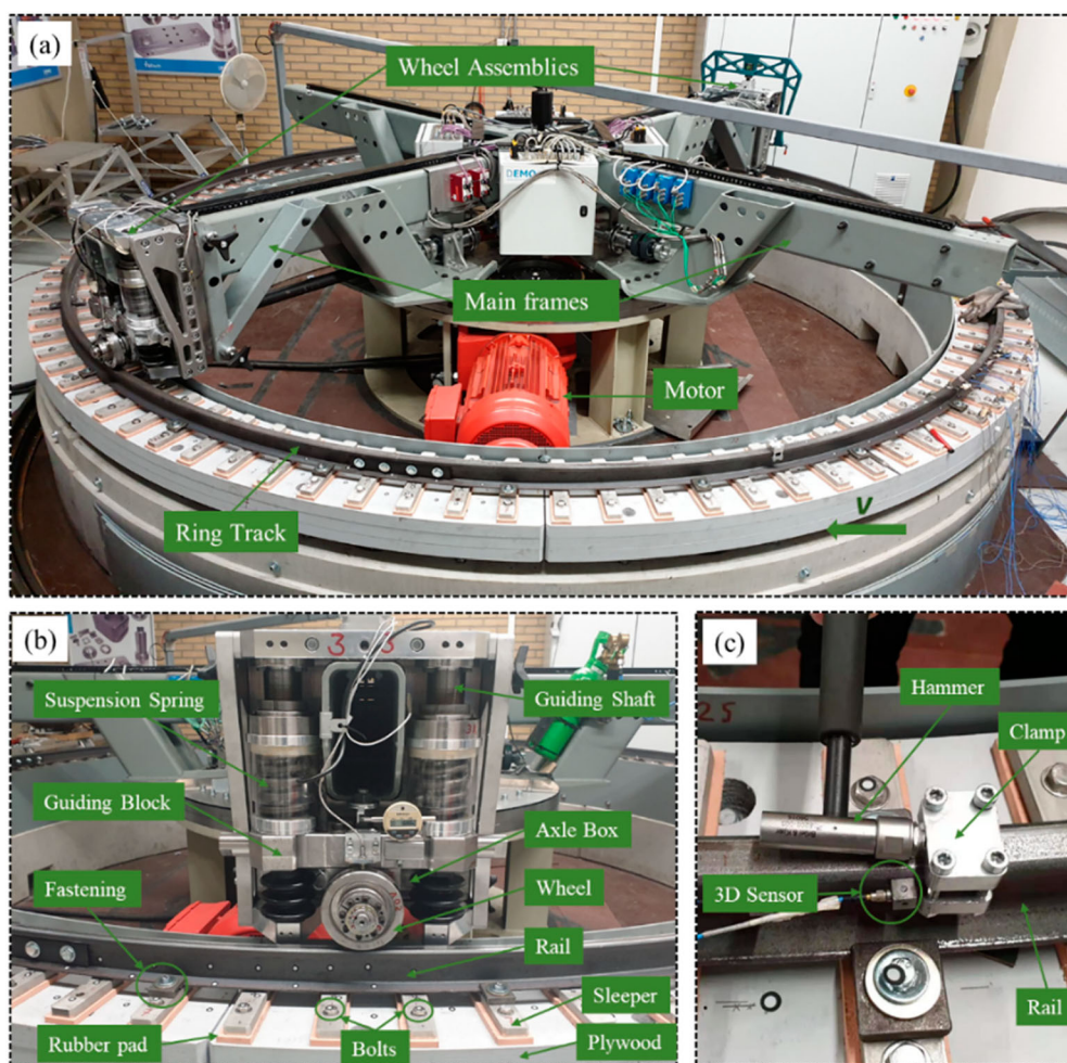
Figure 1. The downscale wheel-rail dynamic interaction test rig named 'V-Track'. (a) Structure of the V-Track, consisting of two wheel assemblies running on a ring track system; (b) main components of the V-Track; (c) setup for the pass-by rail acceleration measurement and the hammer test. The clamp is designed for the longitudinal excitation of the track.
