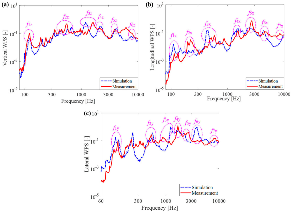
Figure 9. Comparison of simulated and measured rail accelerations in the frequency domain in the (a) vertical, (b) longitudinal, and (c) lateral directions. The dashed pink ovals and corresponding notations ( f_{ix} , f_{iy} , f_{iz} ) indicate the characteristic frequencies of the vehicle-track dynamic interaction in three directions.
