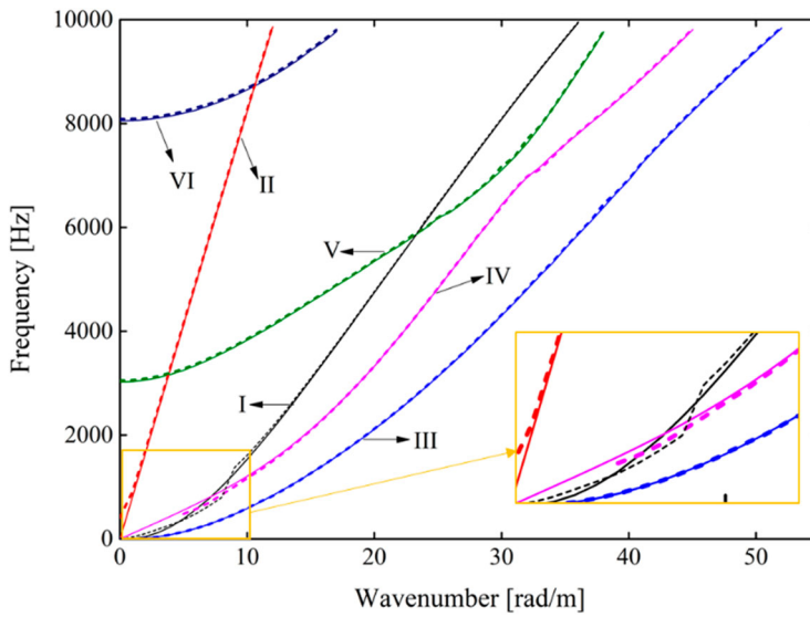
Figure 3. The wavenumber-frequency dispersion relations of the straight (solid lines) and curved (dashed lines) free rail. In this figure, 'I' refers to vertical bending waves, 'II' longitudinal compression waves, 'III' lateral bending waves, 'IV' lateral torsion waves, 'V' web 1st bending waves, and 'VI' web 2nd bending waves. The yellow boxes show the close-up of the results within 2 kHz to better illustrate the difference between the straight and curved rail.
