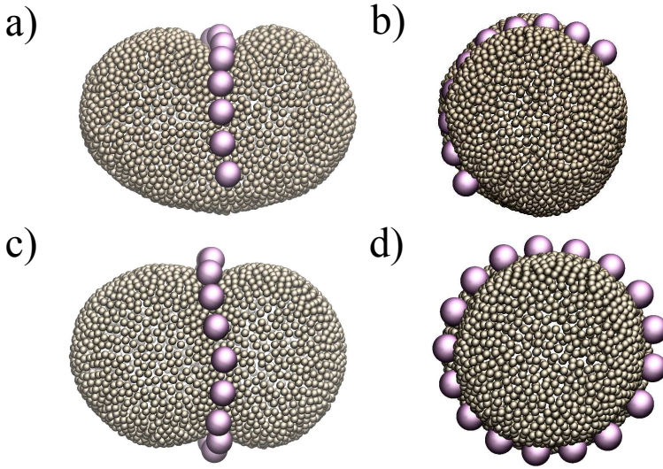
Figure 6.4: Colloids attract each other on ellipsoids, and in order to minimize the curvature energy, they form an arc (a & b) and a ring (c & d) at the mid-plane of the ellipsoid.
