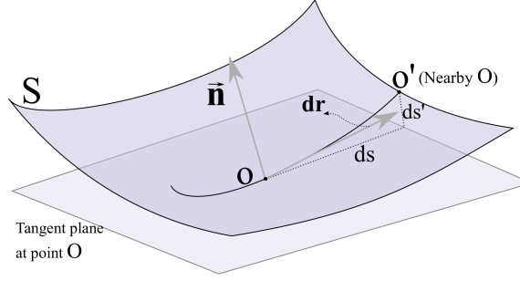
Figure 1.6: The second fundamental form locally characterizes the shape of a surface ( S ) around a point ( O ).
