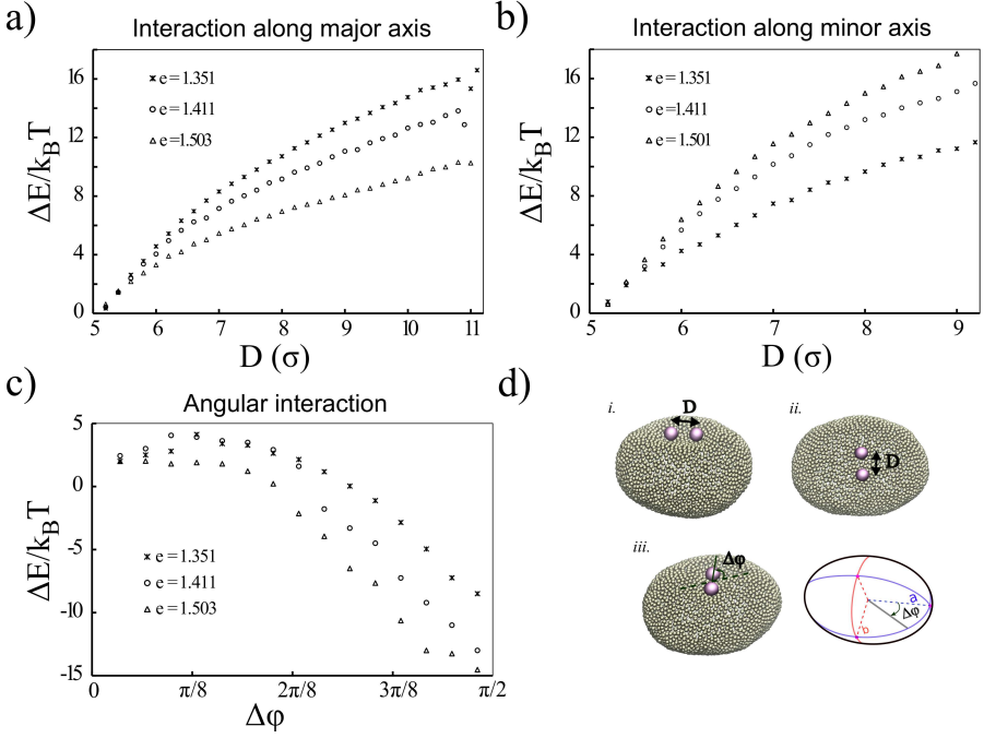
Figure 6.2: Colloids adhered to a quasi-ellipsoidal membrane behave differently in different directions. Decreasing the ellipticity of the vesicle, which is defined as e = a/b , (a) strengthens the attractions between the colloids along the major axis and (b) weakens the interaction between the colloids along the minor axis. Figure (c) illustrates that the energy of a membrane containing a pair of colloids decreases when the angle between the pair and the semi-major axis increases.
