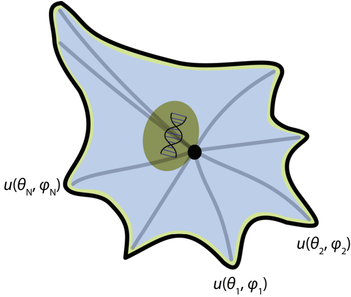
Figure 7.1: Schematic shape of a cell containing some microtubules. We model the microtubules by the imposed deformation ( \tilde{\mathbf{u}}_0 = (u(\theta_1, \phi_1), \dots, u(\theta_N, \phi_N)) ) at their tips.
