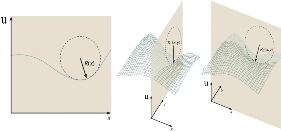
Figure 1.5: The curvature of spatial curves and two dimensional surfaces (From [20]).
