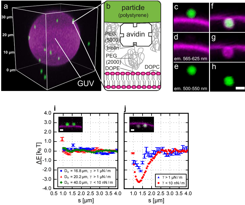
Figure 5.2: Experimental data (a) Three-dimensional confocal image of a typical Giant Unilamellar Vesicle (GUV, in magenta) with attached colloidal particles (in green). (b) Schematic of the avidin-biotin linkage between membrane and particle. By varying the avidin concentration on the particles we control the adhesion strength. Polyethylene glycol (PEG) suppresses electrostatic interactions between membrane and particles, as well as non-specific adhesion between particles. (c) Fluorescence signal of a non-wrapped particle (green) and a membrane (magenta). The separate fluorescence signals of the membrane and particle are displayed in (d,e), respectively. In (f-h) the wrapped state is displayed analogously. (i, j) Interaction energy \Delta E as a function of geodesic particle separation distance s for (i) two non-wrapped particles and (j) two wrapped particles. For non-wrapped particles (i) there is no significant interaction on both tense and floppy membranes. For wrapped particles (j) the interaction potential shows a long-ranged attraction. The scale bars are 1 \mu\text{m} .
