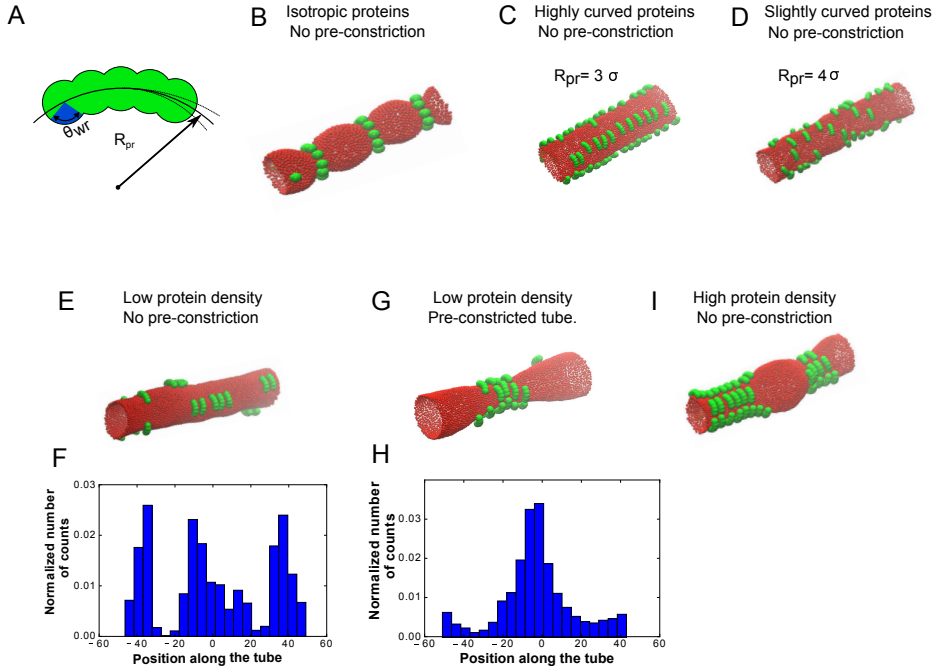
Figure 3.2: Monte Carlo simulation of protein-membrane interactions for different conditions. (A) Proteins were modelled as a linear chain built out of five spheres positioned on a circular arc. Each sphere has a diameter of 4\sigma . (B) Spherical proteins form ring-like structures. (C) Highly curved proteins attracted each other, but only in the longitudinal, and not angular, direction. (D) Slightly curved proteins do not self-assemble at all. In contrast to D and C there is an optimum curvature of proteins for which they attract each other in both angular and longitudinal directions. This requires high density of proteins. (E and F) Proteins with optimum curvature do not exhibit significant collective interaction in low densities. (G and H) In contrast, when the tube is pre-constricted, they sense the region that is under stress and accumulate there. (I) In sufficiently high number, proteins attract each other and constrict the tube (without having pre-constriction).
