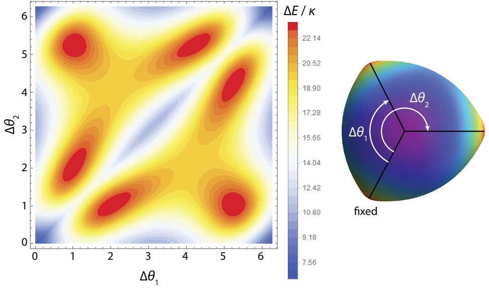
Figure 7.5: Plot of the configuration space of a vesicle with three enclosed microtubules, with the energy of each configuration shown in color. The closed shape of the vesicle favors the formation of parallel structures of microtubules. The global minimum of the energy corresponds to the situation where all the filaments are bundled, with local minima for the case of having two tubules together and one pointing in the opposite direction. Because filaments polymerize from the centrosome in opposite directions, the local minima may be biologically relevant.
