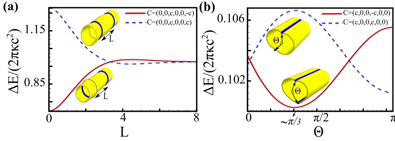
Figure 2.1: The calculated energy cost of having two inclusions (as compared to none) for a membrane tube as a function of the distance between (a) two rings and (b) two rods. Inclusions impose either the same (dashed line) or opposite (solid line) curvatures.
