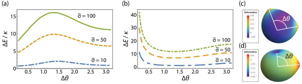
Figure 7.3: The interaction between microtubule-driven protrusions. (a) Microtubules that deform the membrane identically, attract each other and bundle for separations smaller than a critical angle \Delta \theta_c \approx 5\pi/12 . The elastic nature of the membrane hinders microtubule coalescence for larger separations. (b) Protrusions of opposite orientation repel each other for small distances and attract for large angular separations. Right panel: Snapshots of two protrusions that are imposed either identically (c) or oppositely (d).
