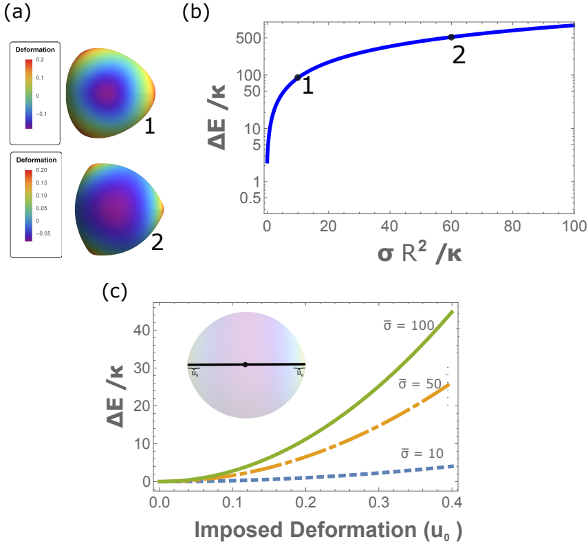
Figure 7.2: Membrane deformation due to the presence of microtubules. (a) Snapshots of a deformed vesicle for low (1) and high (2) values of the surface tension. The imposed deformation vector reads \bar{\mathbf{u}}_0 = (0.1, 0.1, 0.1) . (b) Increasing the in-plane tension makes the membrane deformation more spiky, in contrast to low surface tension regimes where we have rounded deformations. Numbers correspond to the images in (a). (c) The deformation energy of a spherical membrane containing two growing microtubules for different values of the surface tension.
