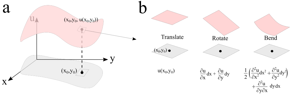
Figure 1.4: (a) Schematic representation of the Monge parametrization. (b) Taylor expansion of the surface u(x, y) around an arbitrary point (From [20]).
