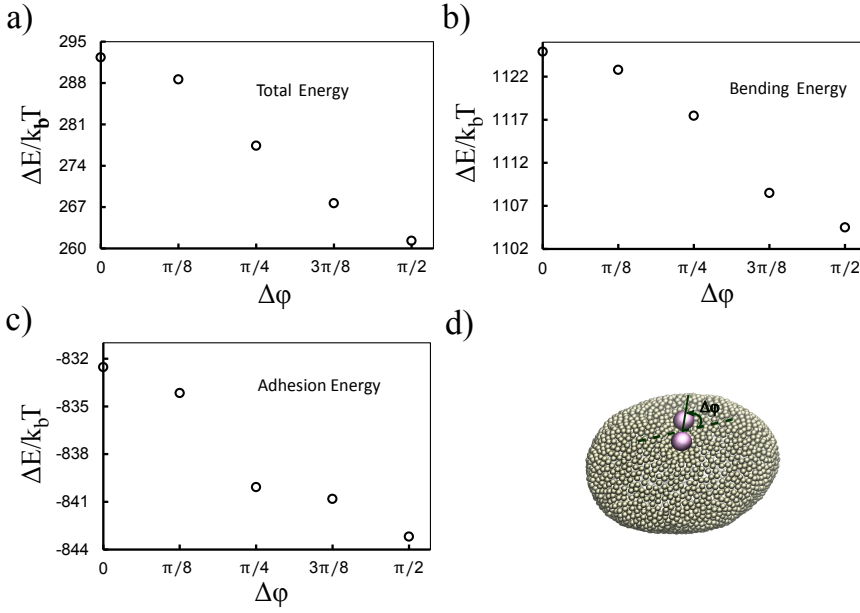
Figure 6.3: Bending is the dominant term in the attraction of colloids. As shown in (b) and (c), both the adhesion energy and the curvature energy are decreasing when the pair of colloids gets aligned with semi-minor axis of the ellipsoid. The latter has a larger contribution in the total energy.
