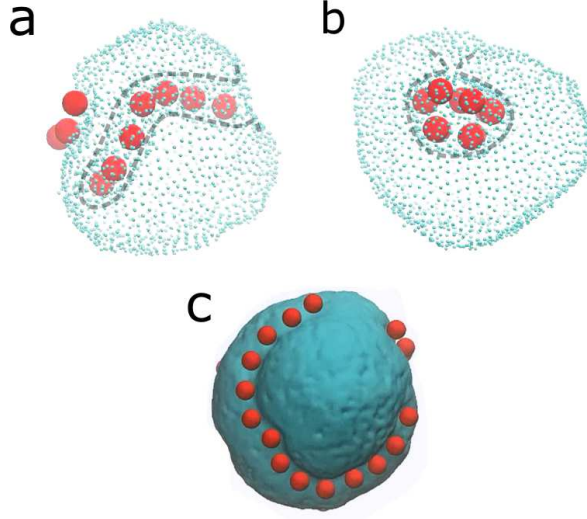
Figure 5.3: Altering the determining constraints relating to the wrapping angle ( \theta_{wr} ), total surface area and enclosed volume leads to completely different collective behaviors. (a and b) There is no conditions on the total surface area and volume of the vesicle, but we only penalize any changes in the surface area. Having fully active particles drives the tubulation of the membrane (a) and partially active particles ( \theta_{wr} = \pi/2 ) collectively induce membrane vesiculation. The adhesion strength and surface tension are set to \varepsilon = 2.8k_B T and \gamma = 1k_B T/\sigma^2 , respectively. (c) Imposing a constant-volume condition drives the formation of linear patterns on the surface of the vesicle.
