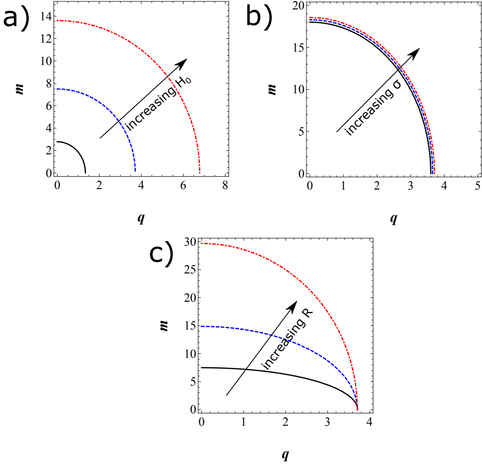
Figure 4.1: Contour plots of the largest eigenvalue \omega_+ of the evolution matrix of our system, as a function of angular and longitudinal modes. For the modes below the plotted contour lines, \omega_+ is positive and the membrane tube becomes unstable. a) Increasing the spontaneous curvature makes the tube more unstable. The black solid, blue dashed and red dashed-dotted lines correspond to H_0 = 0.2 , H_0 = 0.4 and H_0 = 1.2 , respectively. b) Decreasing the surface tension increases (although very slightly) the unstable area. The black solid, blue dashed and red dashed-dotted lines correspond to \sigma = 20 , \sigma = 10 and \sigma = 10/8 , respectively. c) The larger the radius of the tube is, the more unstable the tube becomes in the angular direction. The black solid, blue dashed and red dashed-dotted lines correspond to R = 2 , R = 4 and R = 8 , respectively. In all the cases, \gamma = 1 and \alpha = 1 .
