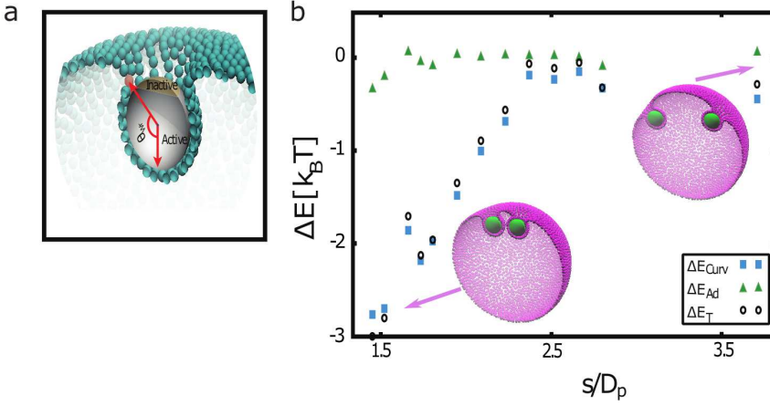
Figure 5.1: Wrapping of particles by the membrane and the resulting total membrane energy in our numerical model. (a) Wrapping happens through adhesion of membrane vertices to colloid particles, due to a strong adhesion potential (Eq. 5.2). We can specify an inactive region at the top of the colloid, preventing the membrane from making very sharp turns (with very high bending energies); in the given example, \theta_{wr} = 11\pi/12 . (b) Curvature, adhesion, and total energy of the system, with zero set at the value of two wrapped particles located at opposite poles of the vesicle. After the wrapping process, the adhesion energy ( \Delta E_{Ad} ) does not change significantly and therefore the curvature energy ( \Delta E_{Curv} ) determines the behaviour of the particles.
