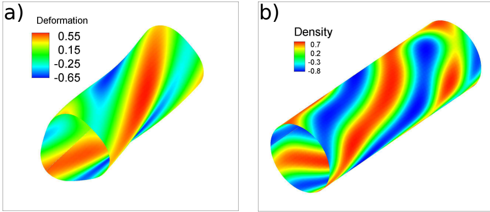
Figure 4.2: The final deformation field (a) and the density of molecules (b) for a membrane started from a state with small random perturbations around u = 0 and \phi = 0 . The relevant parameters are set to H_0 = 0.2 , R = 5 , L = 35 , \gamma = 1 and \alpha = 1 .
