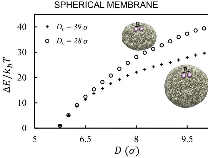
Figure 6.1: Curvature energy of the membrane for spherical vesicles of diameters D_v = 28\sigma (circles) and D_v = 39\sigma (pluses) containing two colloids. The force between colloids in the smaller vesicle is stronger and has a larger interaction range.
