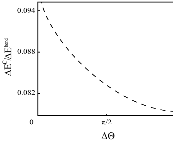
Figure S. 7: Ratio of fluctuation-induced energy to bending energy for an imposed curvature of c = \frac{10}{R} and a bending modulus of \kappa = 25k_B T .
