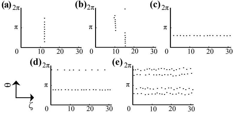
Figure 2.4: Equilibrium configurations obtained by Monte Carlo simulation for a system containing (a) 10 inclusions with hard-core radius of a_0 = 0.2 (b) 16 inclusions with hard-core radius of a_0 = 0.2 (c) 16 inclusions with hard-core radius of a_0 = 1.1 (d) 30 inclusions with hard-core radius of a_0 = 1.1 (e) 80 inclusions with hard-core radius of a_0 = 1.1 .
