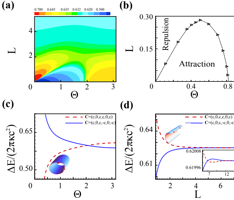
Figure 2.3: (a) The curvature energy ( \frac{\Delta E}{2\pi\kappa c^2} ) of a membrane containing two inclusions, as a function of their angular ( \Theta ) and longitudinal ( L ) separation, with L in units of the tube radius R . (b) The line around the global minimum at which the energy equals the local minimum at large separations. For particles whose diameter exceeds the size of this region, the overall behavior is repulsive (settling in the local minimum at large separations). Smaller particles globally attract, but have a high energy barrier separating the attractive and repulsive regime. (c) Two identical inclusions placed at the same longitudinal coordinates ( L=0 ) attract each other. (d) Point-like inclusions behave like rings when they are situated on the same transversal coordinates ( \Theta=0 ); the inset shows the weak long-range attraction.
