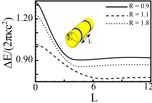
Figure S. 5: The competition between bending modulus and surface tension of the tube determines both the radius of the tube ( R = \sqrt{\kappa/2\sigma} ) and the equilibrium distance between two rings.
