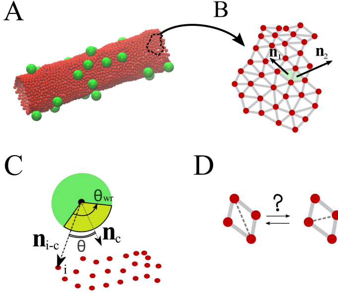
Figure 3.1: We model the membrane tube as composed of many vertices (red beads in (A)) which form a triangulated network (B). Fluidity of membrane is simulated by changing the connection in any two neighboring pairs of triangles (D). In order to study the membrane mediated interactions, we introduce an adhesion force between the colloids (colored in green in (A)) and beads to deform the tube (C). The surface area of every colloid is partitioned into two passive and active (controlled by angle \theta_{wr} ) parts. We found the membrane beads that are exposed to the active part via introducing an angle between the director vector of the active patch ( \mathbf{n}_c ) and the vector connecting the center of the colloid to any arbitrary neighboring bead i ( \mathbf{n}_{i-c} ).
