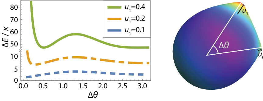
Figure 7.4: Interaction between microtubule-driven protrusions of different strength. As shown in the graph, introducing a difference in the magnitude of the protrusions results in a very strong short range repulsion between them ( u_0 = 0.1 ; \bar{\sigma} = 10 ).
