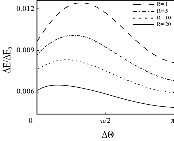
Figure S. 6: In the limit of large radii, the interaction between two rods becomes mostly repulsive, approaching the planar membrane case of pure repulsion.
