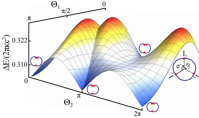
Figure 2.2: The energy landscape for a membrane tube containing three rod like inclusions I1, I2 and I3.
