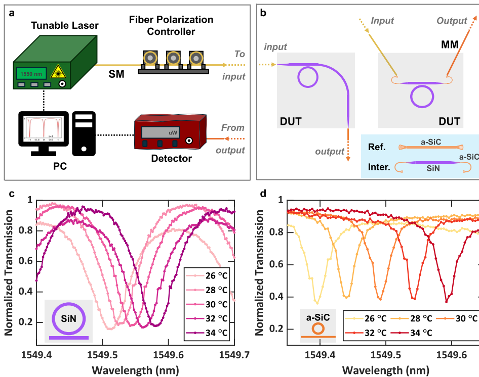
FIG. 1. (a) Characterization setups used to measure the on-chip devices. (b) Two kinds of fiber-to-chip accesses employed in measurements. The blue-background inset illustrates both the interconnection device and the corresponding reference device employed for characterization. [(c) and (d)] Thermo-optic characterization of the a-SiC/SiN platform: the resonance shifts observed when sweeping the temperature from 26 to 34 °C on the SiN ring resonator and a-SiC ring resonator, respectively.
