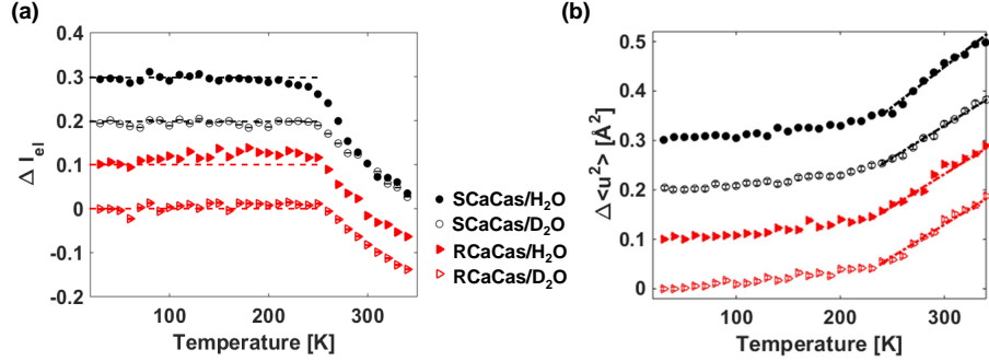
Figure 3: (a): Change of the elastic incoherent intensity \Delta I_{el} as a function of temperature. (b): MSDs of the hydrated samples as a function of temperature. For clarity, the plots of RCaCas hydrated with H 2 O (filled triangle), SCaCas hydrated with D 2 O (hollow circle) and H 2 O (filled circle) are shifted by 0.1, 0.2 and 0.3, respectively. The dashed lines are guides to the eye.
