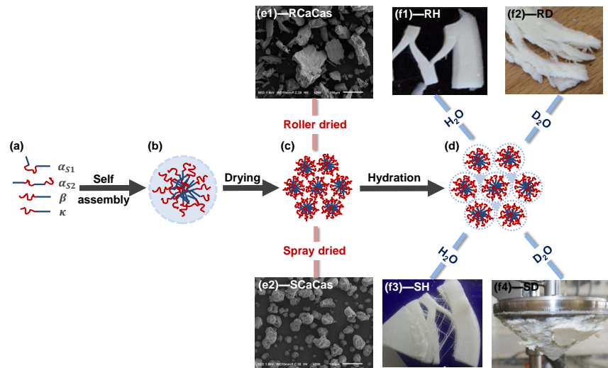
Figure 4: Schematic illustration of the status of the calcium caseinate aggregates from solution (a-b) to dried powders (c&e) and to re-hydration with different solvents (d&f). (a): the four sub-caseins are depicted according to the Horne. et al [47], where the straight lines represent the hydrophobic region and the twisting lines represent the hydrophilic region. (b): a simplified depiction of one micelle-like aggregate in solution before drying, based on the model from the de Kruif [27]. Note, Ca^{2+} ions distribute homogeneously inside the aggregates, but are not shown in the drawing since they are not the interest of this discussion. (c): after drying, the micelle-like aggregates collapse into bigger aggregates that form the powder particle. (d): after hydration, each individual aggregate is surrounded by a thin layer of solvent (blue dashed lines), with some free solvent dispersed in between (blue triangle). (e): Scanning electron microscopy images of dried RCaCas (e1) and SCaCas (e2) powders. (f1-2): pictures of RCaCas gels made with H_2O and D_2O ; (f3-4): pictures of SCaCas gels made with H_2O and D_2O .
