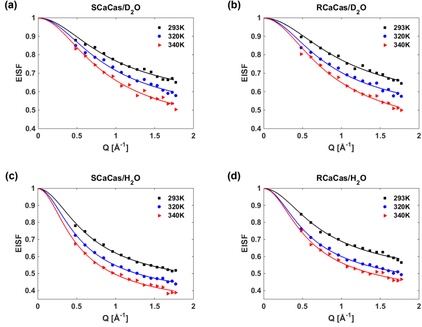
Figure 2: EISF fitted with the free diffusion in a sphere model, plotted as a function of Q at different temperatures. SCaCas and RCaCas powders are hydrated with D_2O (a-b) or H_2O (c-d).
