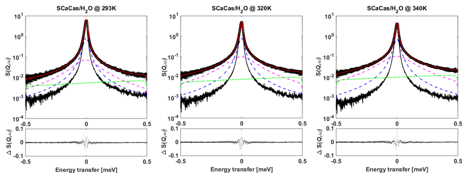
Figure 1: From left to right: QENS spectra of SCaCas powder hydrated with H 2 O measured at 293 K, 320 K and 340 K. The residuals are plotted underneath, they are calculated as the difference between the measured and fitted S(Q, \omega) . The delta function is represented by the black dots, the two Lorentzians are dashed lines in blue and magenta, the background is dash-dot line in green, and the total fitted curve is represented by the red line.
