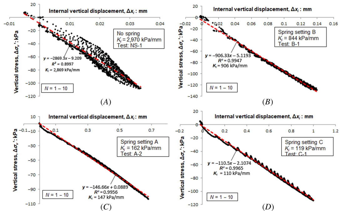
FIG. 14 Relationship between internal vertical displacement, \Delta x_i , and effective vertical stress reduction, \Delta \sigma'_v , during LVDT controlled cyclic loading of dense Toyoura sand samples performed on apparatus DSS A at D_r \sim 80\% and \tau_{xy} = \pm 20 kPa. Test results for (A) no springs, test NS-1; (B) spring setting B, test B-1; (C) spring setting A, test A-2; (D) spring setting C, test C-1.
