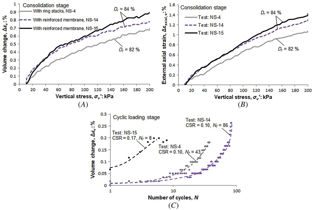
FIG. 16 Variation in (A) volume change, \Delta\epsilon_v , and (B) external axial strain, \Delta\epsilon_{axial, e} , with effective vertical stress, \sigma'_v , during consolidation; (C) relation between volume change, \Delta\epsilon_v , and number of cycles, N , during cyclic loading of LVDT-controlled dense Toyoura sand samples performed on apparatus DSS A.
