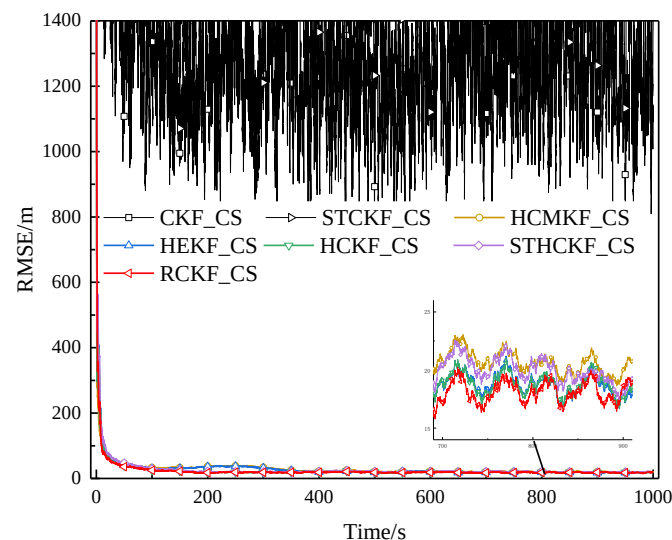
Figure 22. RMSE of example 1 in surface track 1 (Experiment B).
