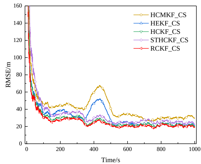
Figure 26. RMSE of example 2 in surface track 2 (Experiment B).
