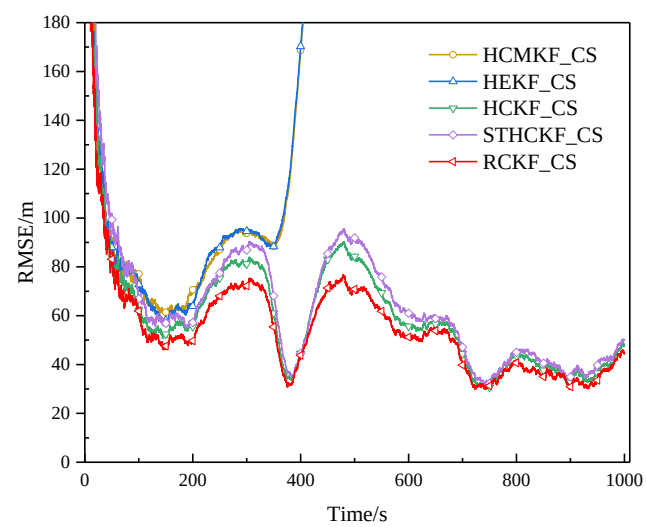
Figure 28. RMSE of example 1 in surface track 3 (Experiment B).
