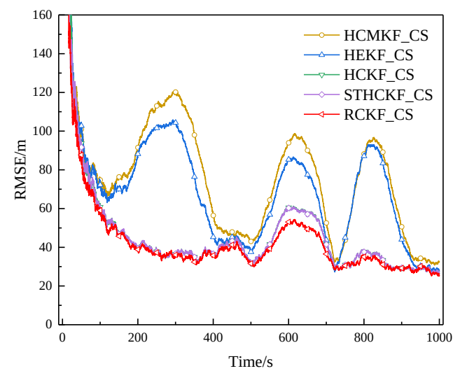
Figure 15. RMSE of example 1 in surface track 4 (Experiment A).
