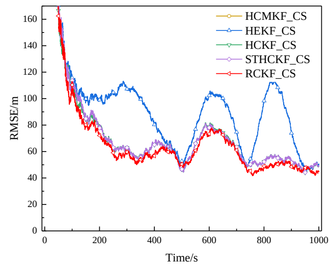
Figure 17. RMSE of example 3 in surface track 4 (Experiment A).
