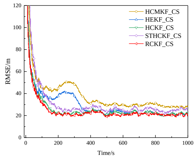
Figure 23. RMSE of example 2 in surface track 1 (Experiment B).
