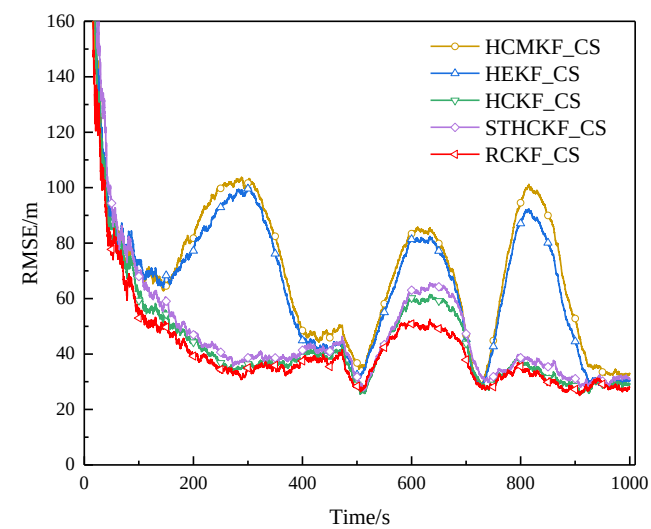
Figure 31. RMSE of example 1 in surface track 4 (Experiment B).
