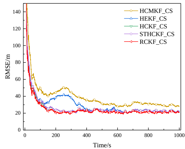
Figure 7. RMSE of example 2 in surface track 1 (Experiment A).
