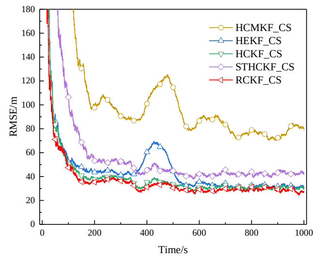
Figure 27. RMSE of example 3 in surface track 2 (Experiment B).
