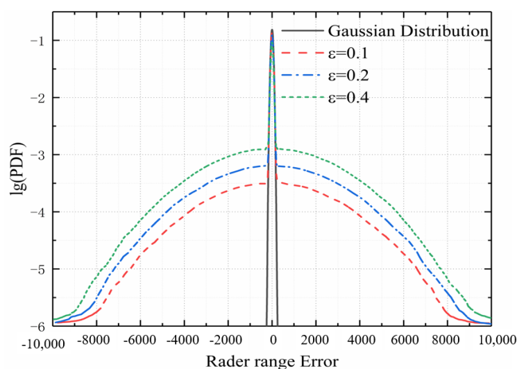
Figure 4. The lg (PDF) of glint noise of Experiment A.
