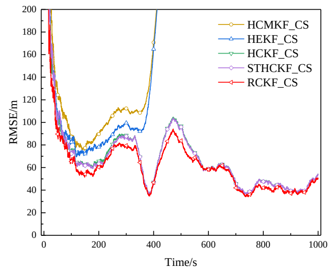
Figure 13. RMSE of example 2 in surface track 3 (Experiment A).
