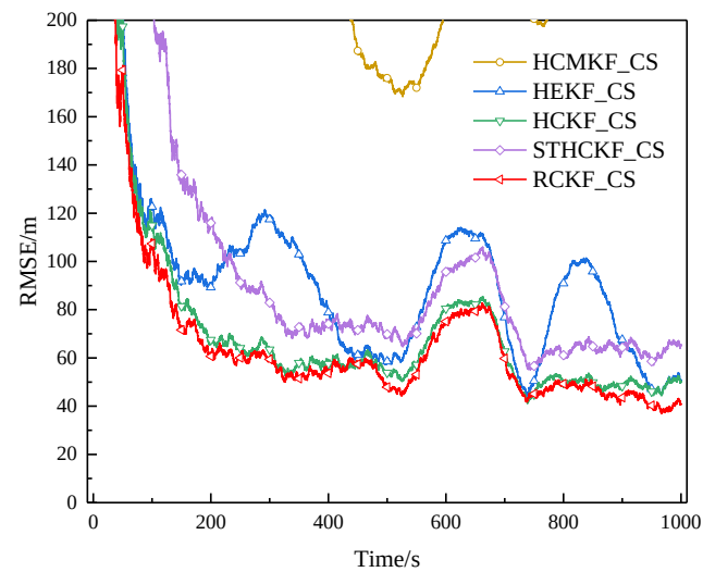
Figure 33. RMSE of example 3 in surface track 4 (Experiment B).
