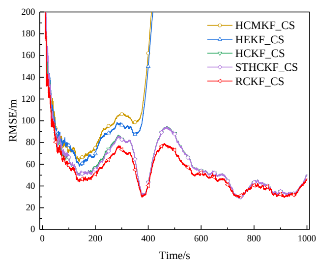
Figure 12. RMSE of example 1 in surface track 3 (Experiment A).
