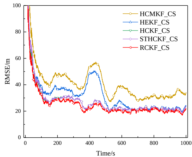
Figure 10. RMSE of example 2 in surface track 2 (Experiment A).
