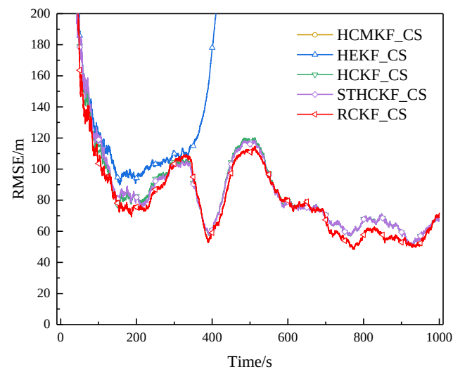
Figure 14. RMSE of example 3 in surface track 3 (Experiment A).
