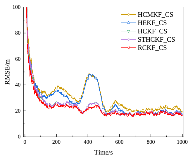
Figure 9. RMSE of example 1 in surface track 2 (Experiment A).
