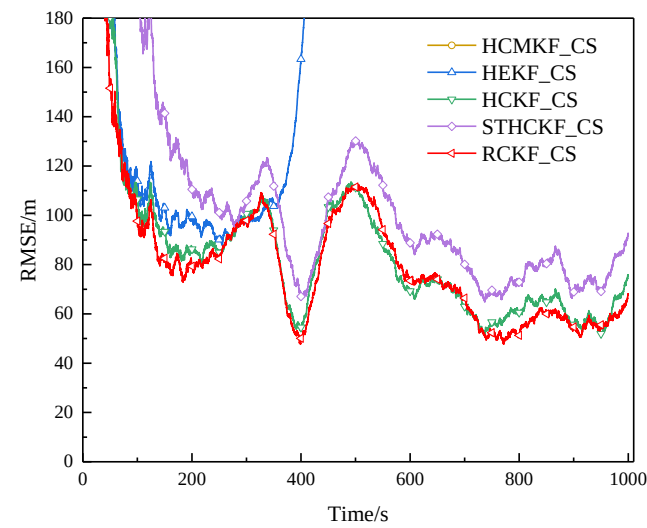
Figure 30. RMSE of example 3 in surface track 3 (Experiment B).
