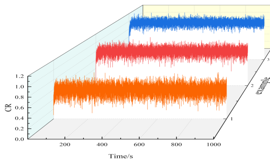
Figure 34. Condition number ratio curve of surface track 1 (Experiment B).
