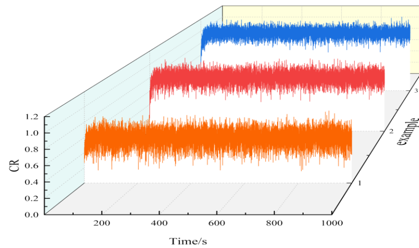
Figure 36. Condition number ratio curve of surface track 3 (Experiment B).
