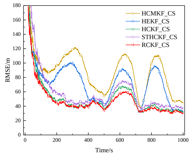
Figure 32. RMSE of example 2 in surface track 4 (Experiment B).
