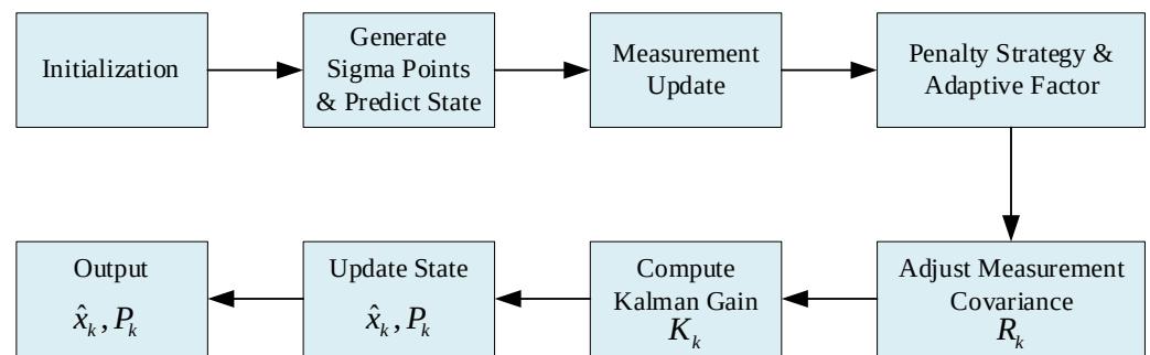
Figure 1. Flowchart of the proposed RCKF_CS algorithm illustrating the key steps.
