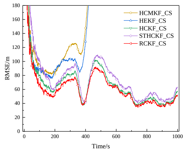
Figure 29. RMSE of example 2 in surface track 3 (Experiment B).
