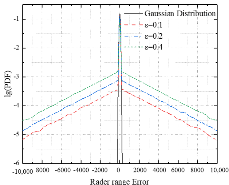
Figure 5. The lg (PDF) of glint noise of Experiment B.
