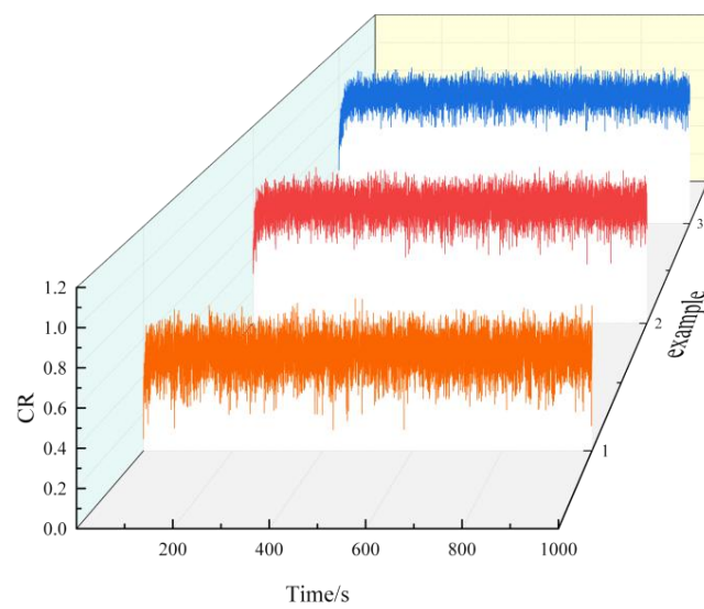
Figure 21. Condition number ratio curve of surface track 4 (Experiment A).
