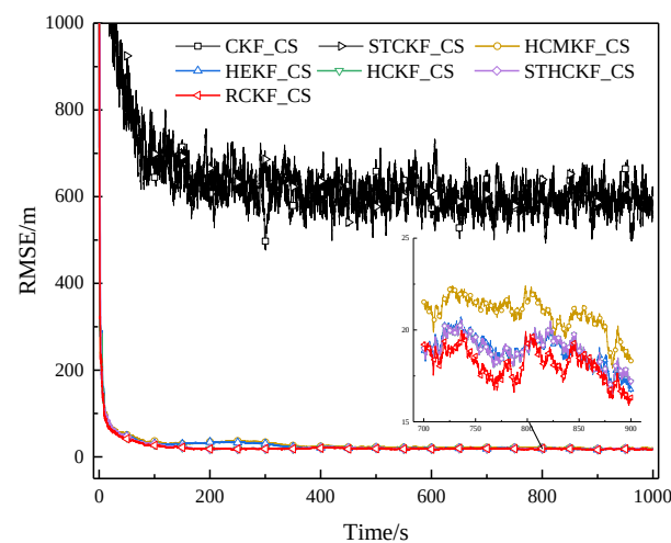
Figure 6. RMSE of example 1 in surface track 1 (Experiment A).
