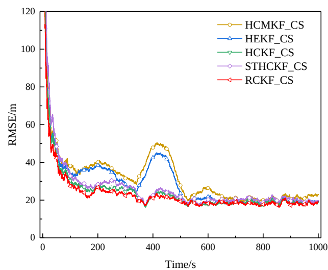
Figure 25. RMSE of example 1 in surface track 2 (Experiment B).
