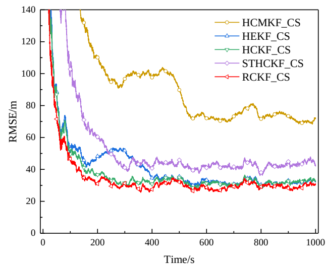
Figure 24. RMSE of example 3 in surface track 1 (Experiment B).
