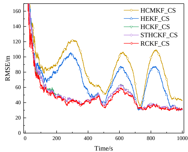
Figure 16. RMSE of example 2 in surface track 4 (Experiment A).
