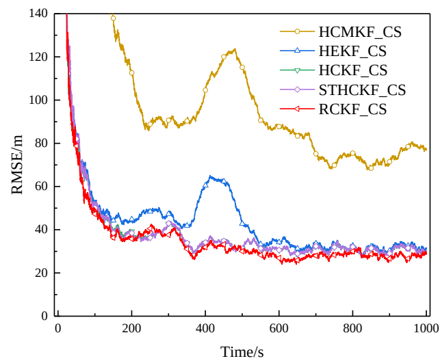
Figure 11. RMSE of example 3 in surface track 2 (Experiment A).
