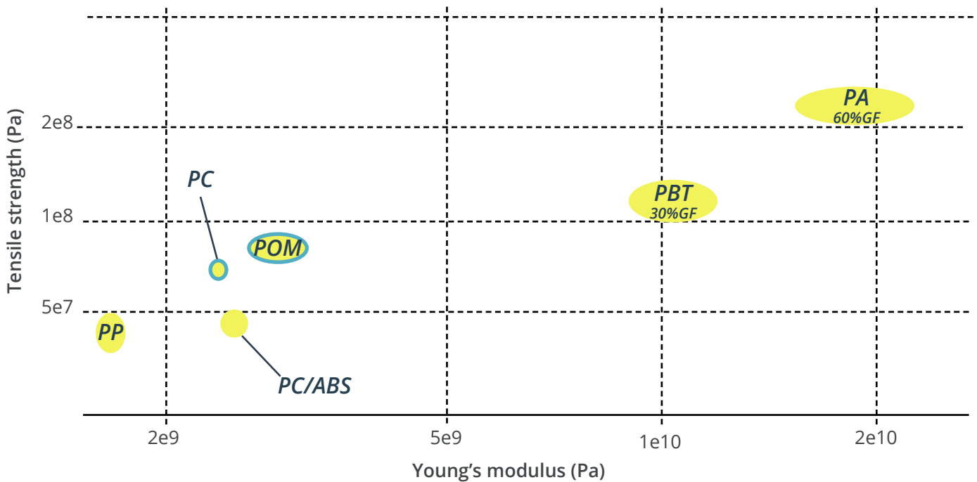
Figure 41 Young's modulus, Tensile strength, CES edupack 2022
