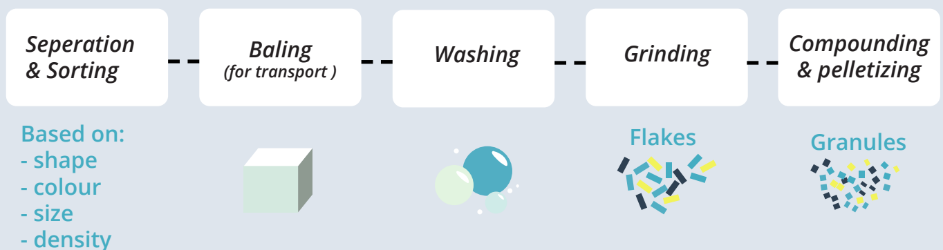
Figure 13 Mechanical recycling process
