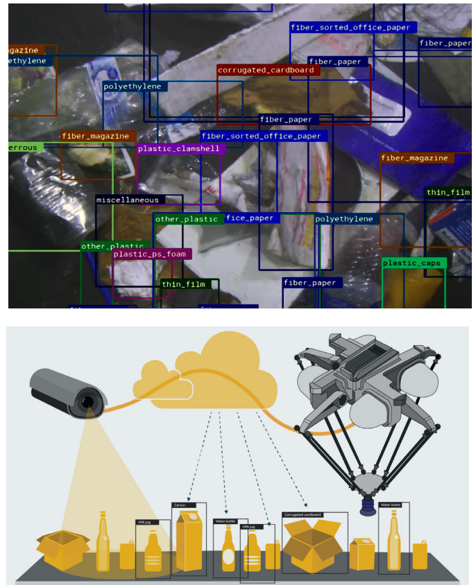
Figure 15 AMP Robotics (2021), AI driven sorting system
