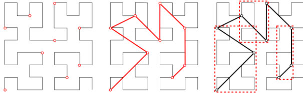
Figure 4: Two-dimensional schematic example of sorting and grouping objects according to their centroid using a SFC.
